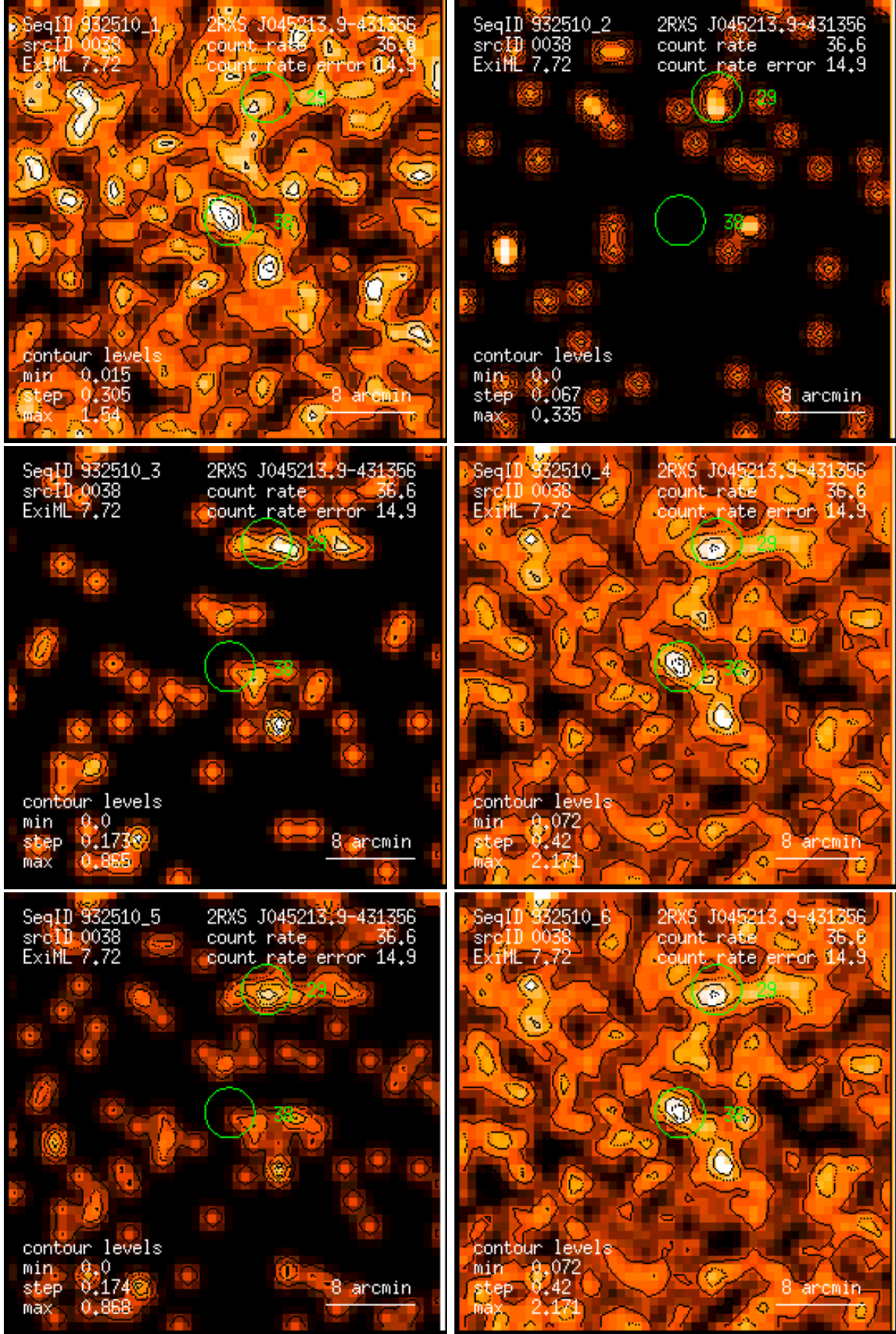
Figure 38: RASS 932510: detection 0038: band rate images, Gaussian filter: (1) PSPC channels 11 – 41, (2) 52 – 90, (3) 91 – 201, (4) 11 – 235, (5) 52 – 201, (6) 11 – 201. Broad band rates in counts/ks. Band rate contour levels in counts/ks/arcmin 2 .
