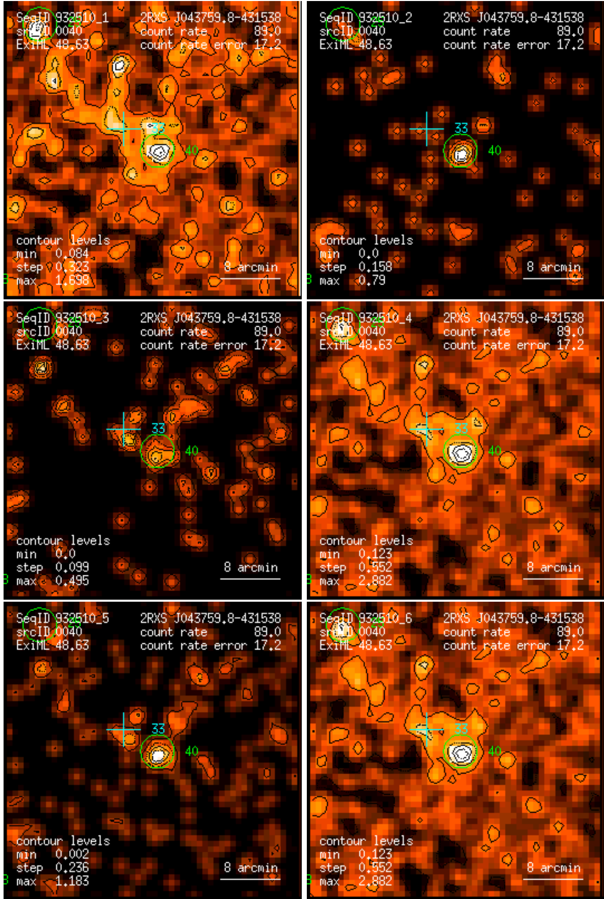
Figure 40: RASS 932510: detection 0040: band rate images, Gaussian filter: (1) PSPC channels 11 – 41, (2) 52 – 90, (3) 91 – 201, (4) 11 – 235, (5) 52 – 201, (6) 11 – 201. Broad band rates in counts/ks. Band rate contour levels in counts/ks/arcmin 2 .
