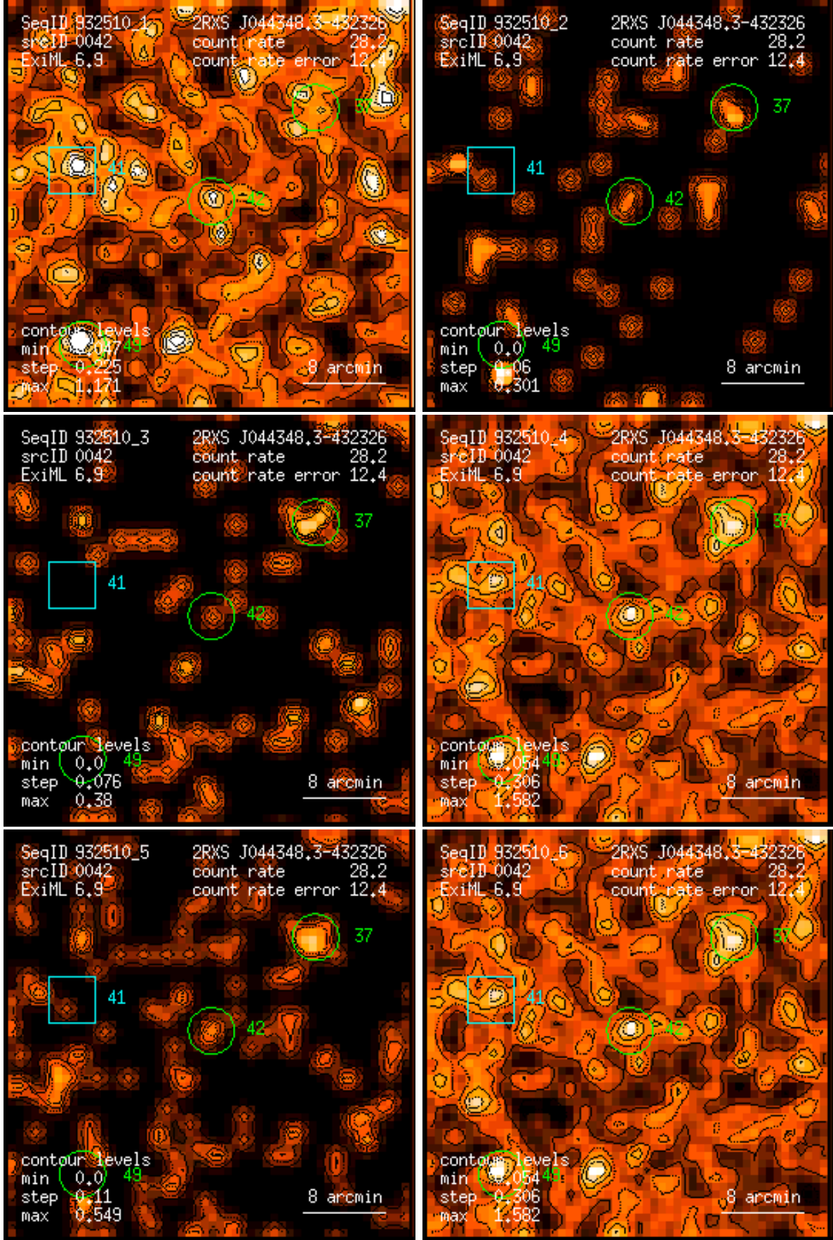
Figure 42: RASS 932510: detection 0042: band rate images, Gaussian filter: (1) PSPC channels 11 – 41, (2) 52 – 90, (3) 91 – 201, (4) 11 – 235, (5) 52 – 201, (6) 11 – 201. Broad band rates in counts/ks. Band rate contour levels in counts/ks/arcmin 2 .
