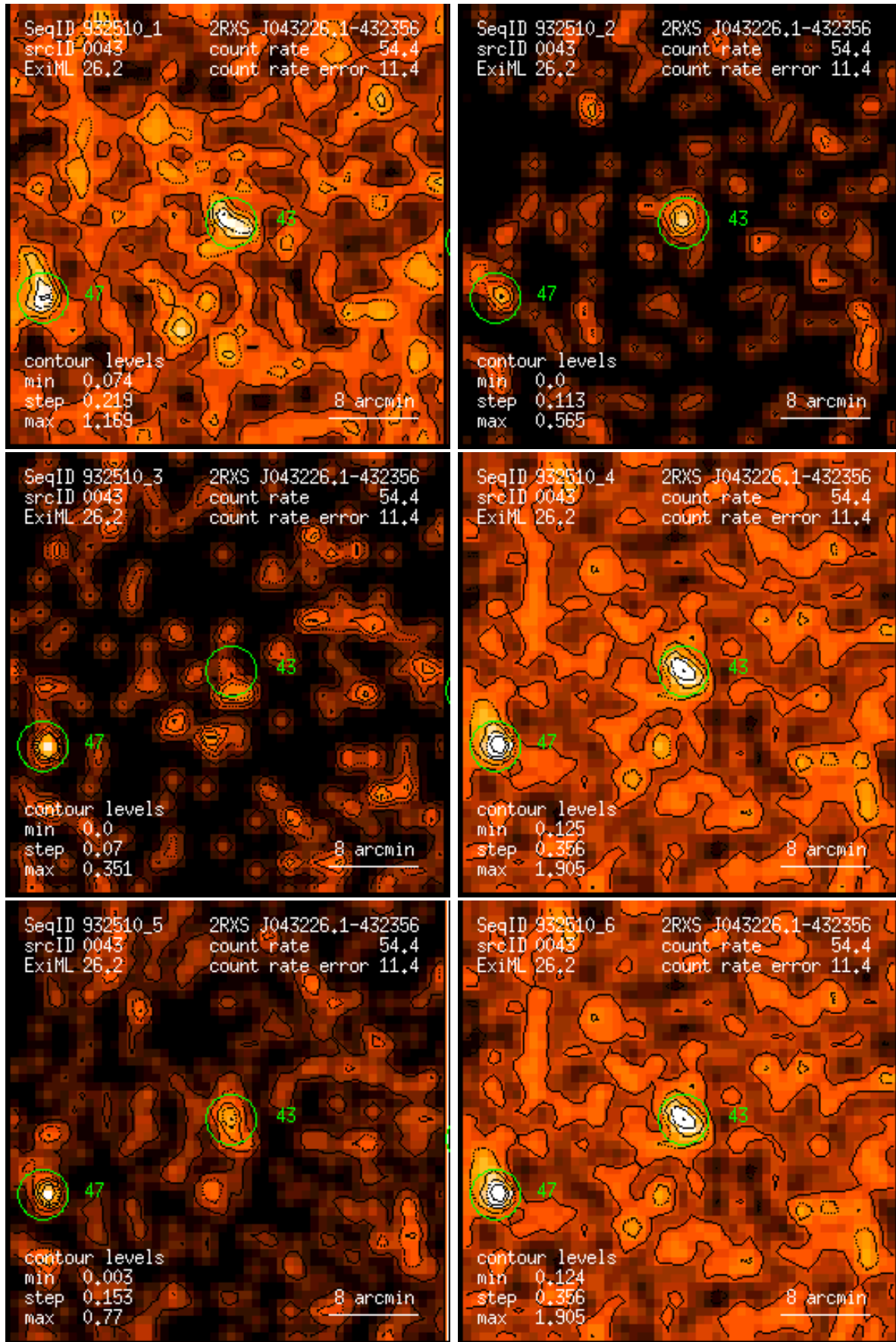
Figure 43: RASS 932510: detection 0043: band rate images, Gaussian filter: (1) PSPC channels 11 – 41, (2) 52 – 90, (3) 91 – 201, (4) 11 – 235, (5) 52 – 201, (6) 11 – 201. Broad band rates in counts/ks. Band rate contour levels in counts/ks/arcmin 2 .
