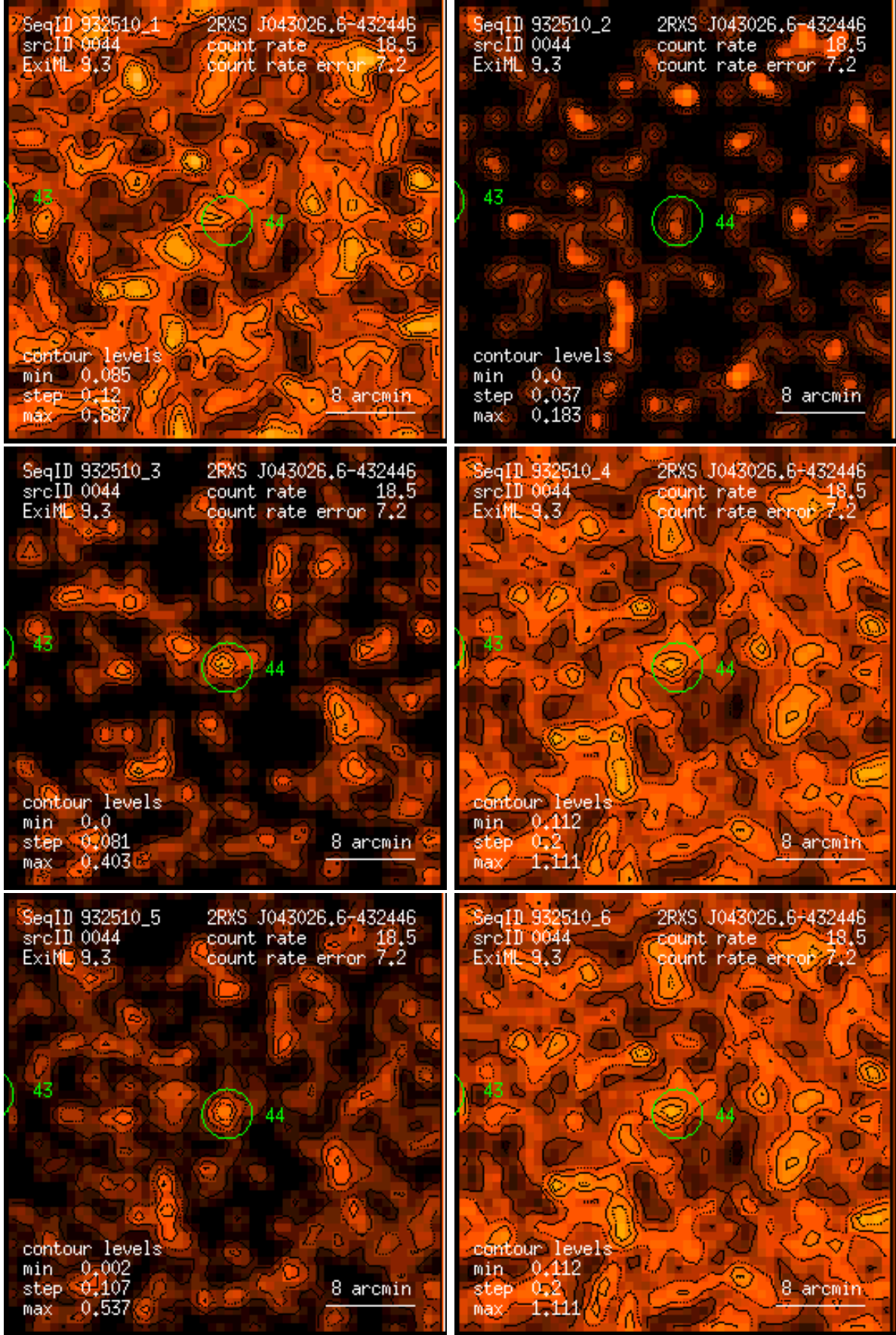
Figure 44: RASS 932510: detection 0044: band rate images, Gaussian filter: (1) PSPC channels 11 – 41, (2) 52 – 90, (3) 91 – 201, (4) 11 – 235, (5) 52 – 201, (6) 11 – 201. Broad band rates in counts/ks. Band rate contour levels in counts/ks/arcmin 2 .
