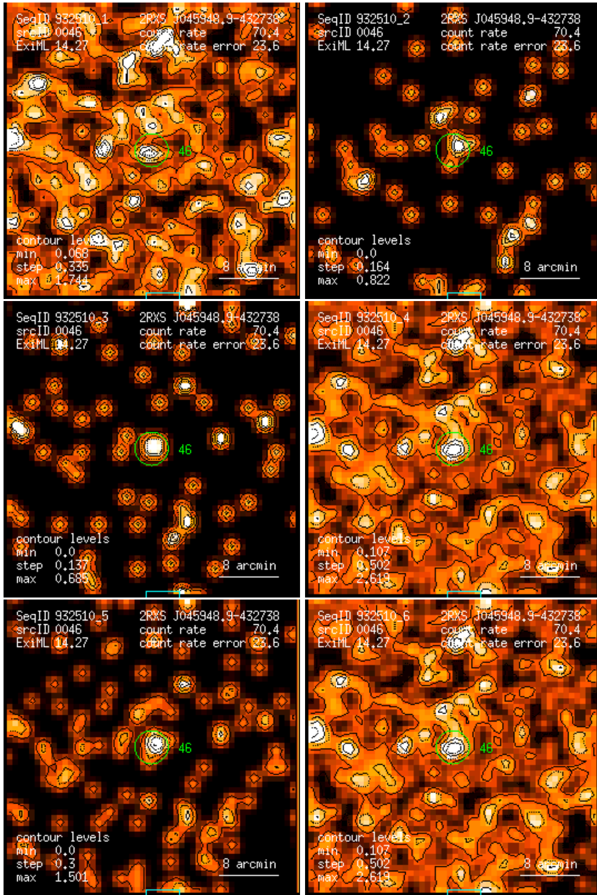
Figure 46: RASS 932510: detection 0046: band rate images, Gaussian filter: (1) PSPC channels 11 – 41, (2) 52 – 90, (3) 91 – 201, (4) 11 – 235, (5) 52 – 201, (6) 11 – 201. Broad band rates in counts/ks. Band rate contour levels in counts/ks/arcmin 2 .
