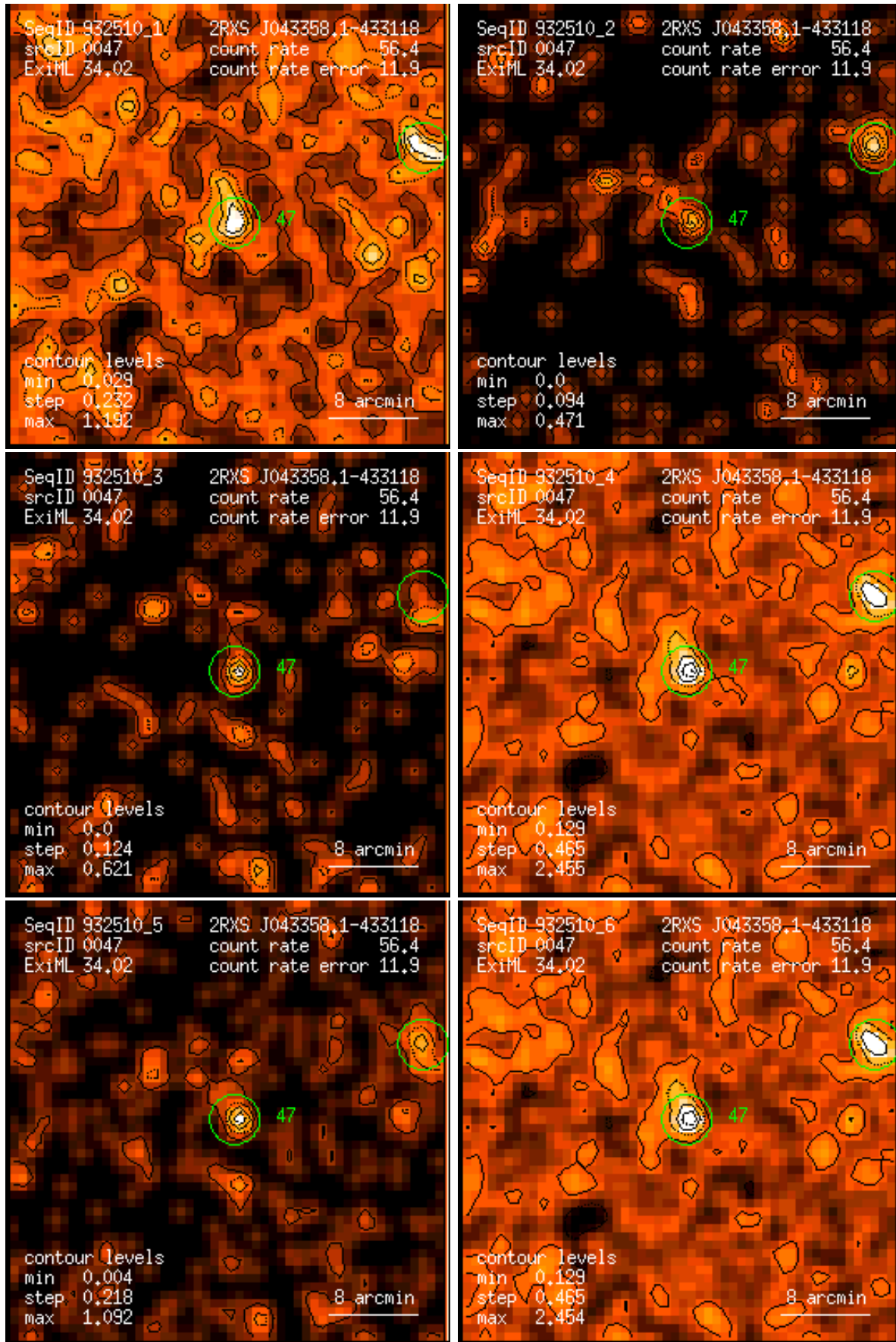
Figure 47: RASS 932510: detection 0047: band rate images, Gaussian filter: (1) PSPC channels 11 – 41, (2) 52 – 90, (3) 91 – 201, (4) 11 – 235, (5) 52 – 201, (6) 11 – 201. Broad band rates in counts/ks. Band rate contour levels in counts/ks/arcmin 2 .
