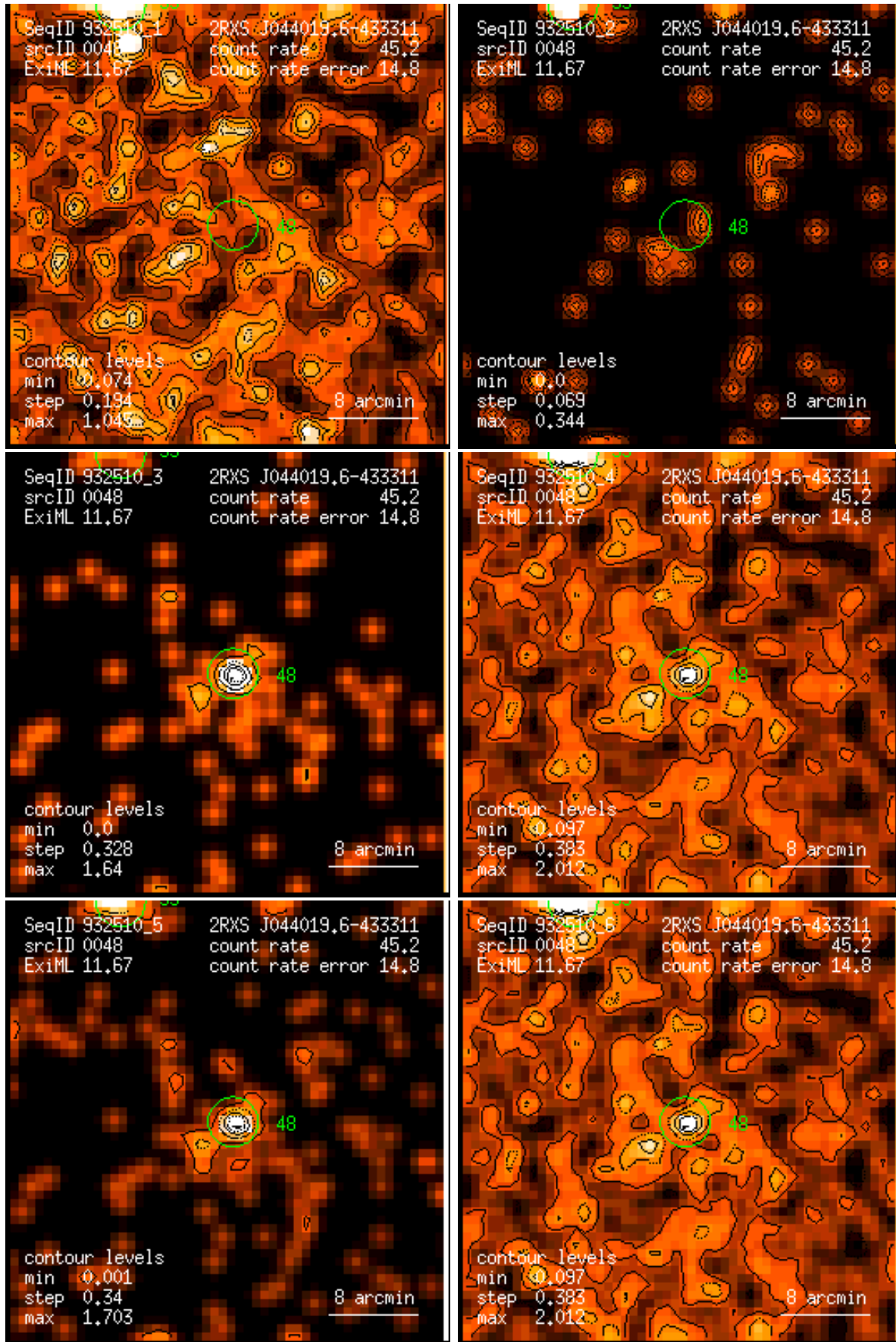
Figure 48: RASS 932510: detection 0048: band rate images, Gaussian filter: (1) PSPC channels 11 – 41, (2) 52 – 90, (3) 91 – 201, (4) 11 – 235, (5) 52 – 201, (6) 11 – 201. Broad band rates in counts/ks. Band rate contour levels in counts/ks/arcmin 2 .
