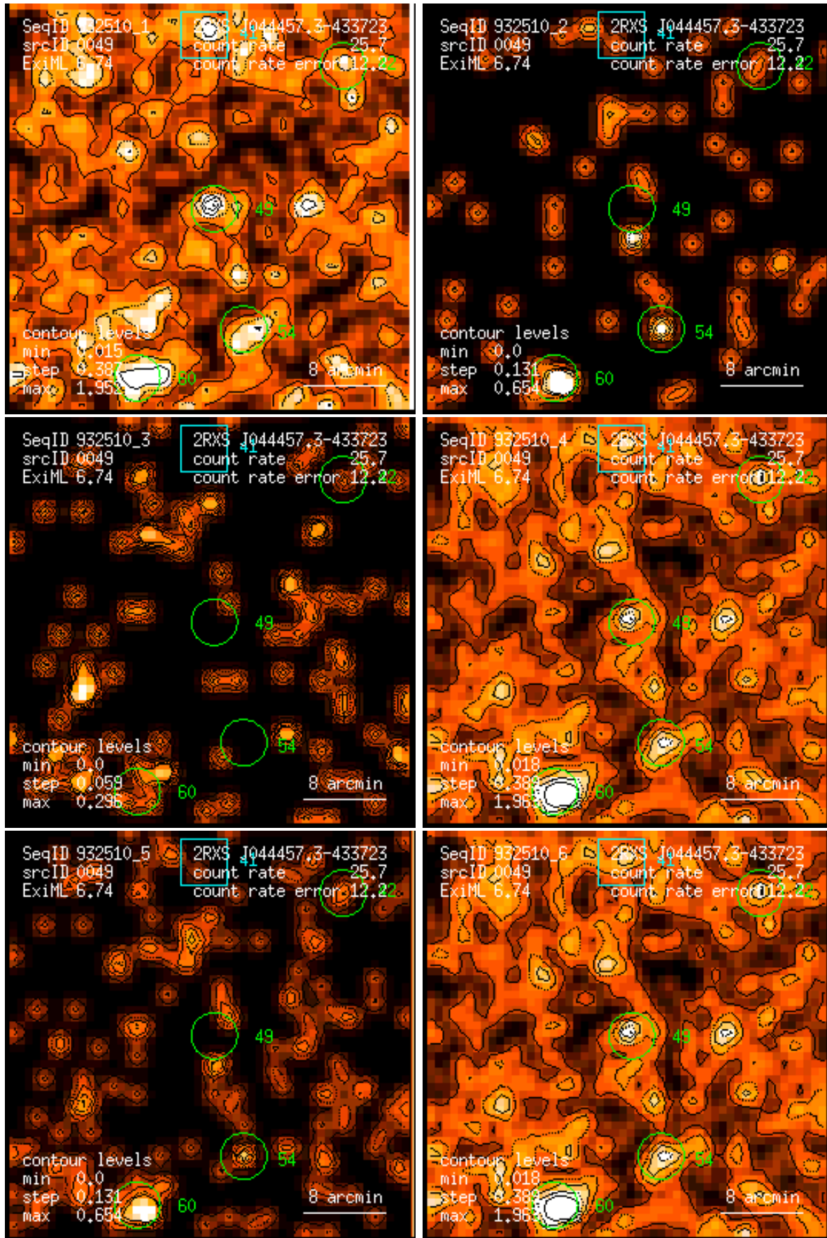
Figure 49: RASS 932510: detection 0049: band rate images, Gaussian filter: (1) PSPC channels 11 – 41, (2) 52 – 90, (3) 91 – 201, (4) 11 – 235, (5) 52 – 201, (6) 11 – 201. Broad band rates in counts/ks. Band rate contour levels in counts/ks/arcmin 2 .
