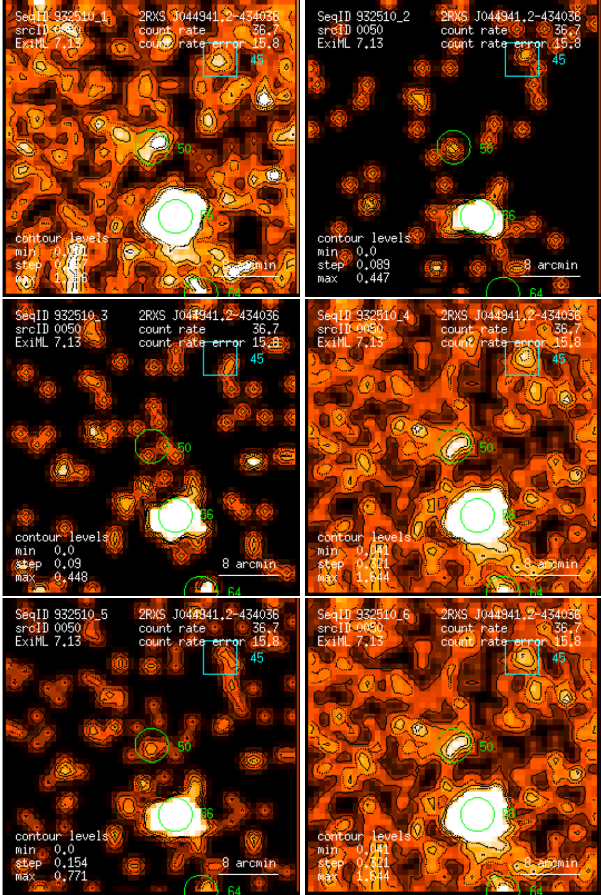
Figure 50: RASS 932510: detection 0050: band rate images, Gaussian filter: (1) PSPC channels 11 – 41, (2) 52 – 90, (3) 91 – 201, (4) 11 – 235, (5) 52 – 201, (6) 11 – 201. Broad band rates in counts/ks. Band rate contour levels in counts/ks/arcmin 2 .
