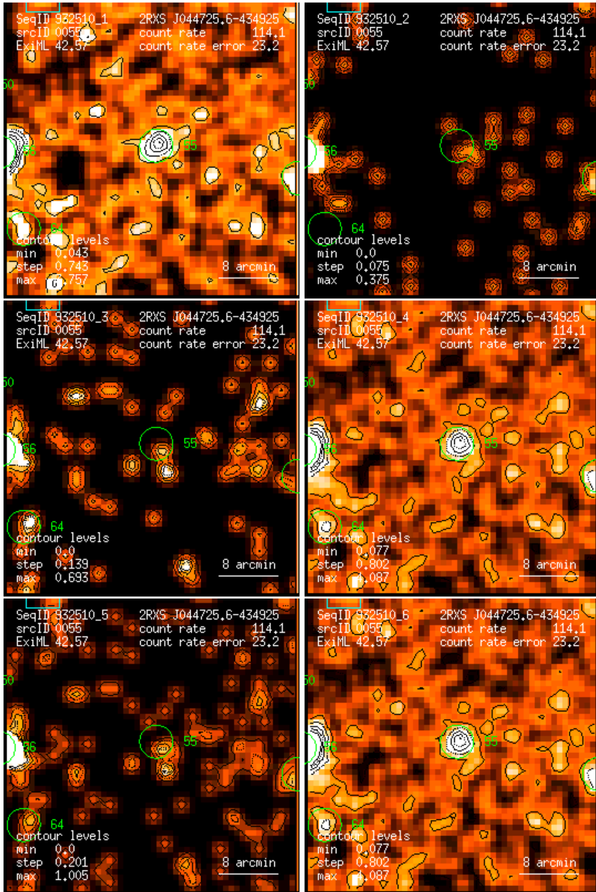
Figure 55: RASS 932510: detection 0055: band rate images, Gaussian filter: (1) PSPC channels 11 – 41, (2) 52 – 90, (3) 91 – 201, (4) 11 – 235, (5) 52 – 201, (6) 11 – 201. Broad band rates in counts/ks. Band rate contour levels in counts/ks/arcmin 2 .
