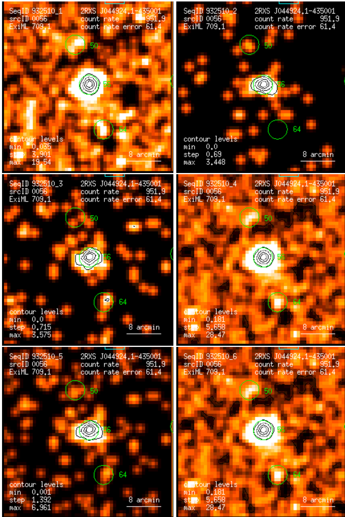
Figure 56: RASS 932510: detection 0056: band rate images, Gaussian filter: (1) PSPC channels 11 – 41, (2) 52 – 90, (3) 91 – 201, (4) 11 – 235, (5) 52 – 201, (6) 11 – 201. Broad band rates in counts/ks. Band rate contour levels in counts/ks/arcmin 2 .
