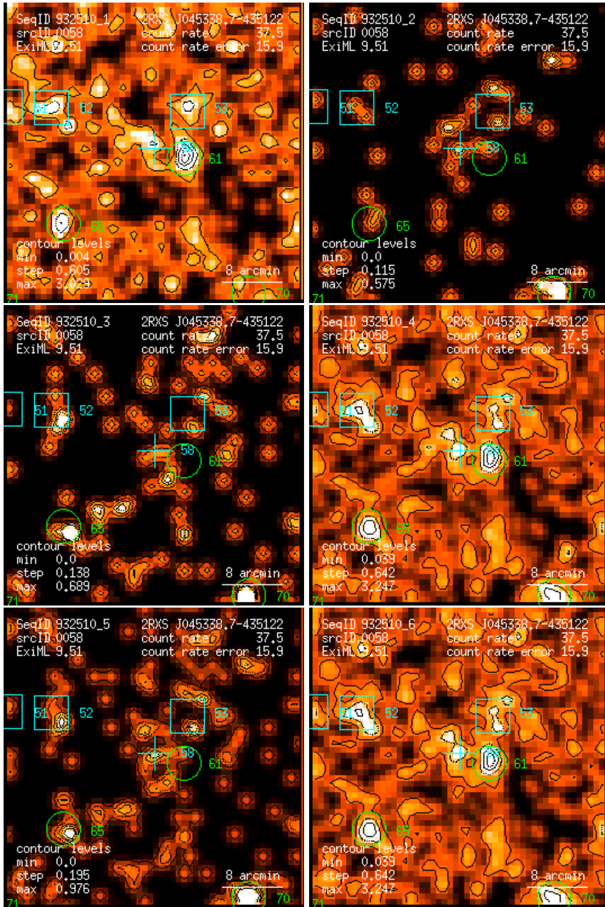
Figure 58: RASS 932510: detection 0058: band rate images, Gaussian filter: (1) PSPC channels 11 – 41, (2) 52 – 90, (3) 91 – 201, (4) 11 – 235, (5) 52 – 201, (6) 11 – 201. Broad band rates in counts/ks. Band rate contour levels in counts/ks/arcmin 2 .
