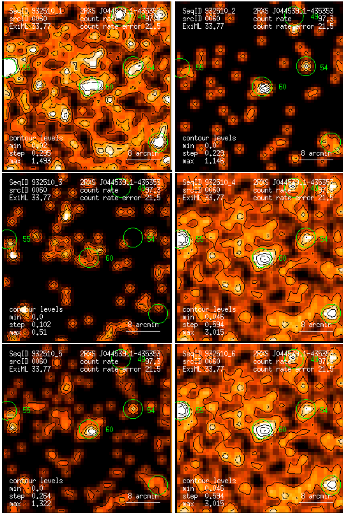
Figure 60: RASS 932510: detection 0060: band rate images, Gaussian filter: (1) PSPC channels 11 – 41, (2) 52 – 90, (3) 91 – 201, (4) 11 – 235, (5) 52 – 201, (6) 11 – 201. Broad band rates in counts/ks. Band rate contour levels in counts/ks/arcmin 2 .
