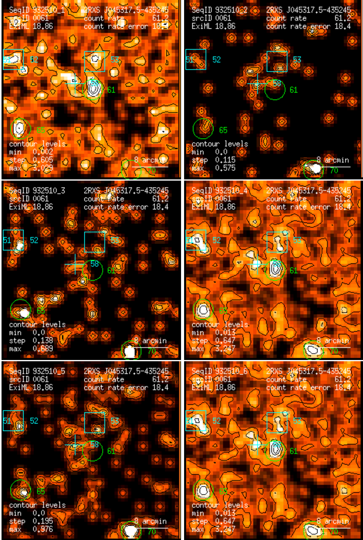
Figure 61: RASS 932510: detection 0061: band rate images, Gaussian filter: (1) PSPC channels 11 – 41, (2) 52 – 90, (3) 91 – 201, (4) 11 – 235, (5) 52 – 201, (6) 11 – 201. Broad band rates in counts/ks. Band rate contour levels in counts/ks/arcmin 2 .
