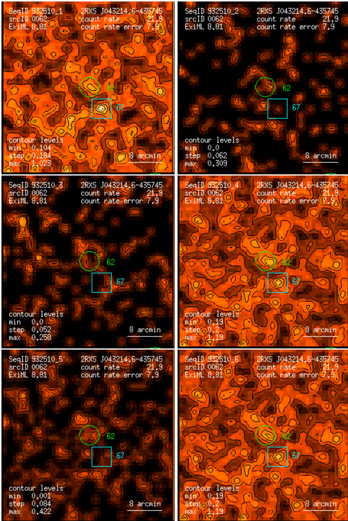
Figure 62: RASS 932510: detection 0062: band rate images, Gaussian filter: (1) PSPC channels 11 – 41, (2) 52 – 90, (3) 91 – 201, (4) 11 – 235, (5) 52 – 201, (6) 11 – 201. Broad band rates in counts/ks. Band rate contour levels in counts/ks/arcmin 2 .
