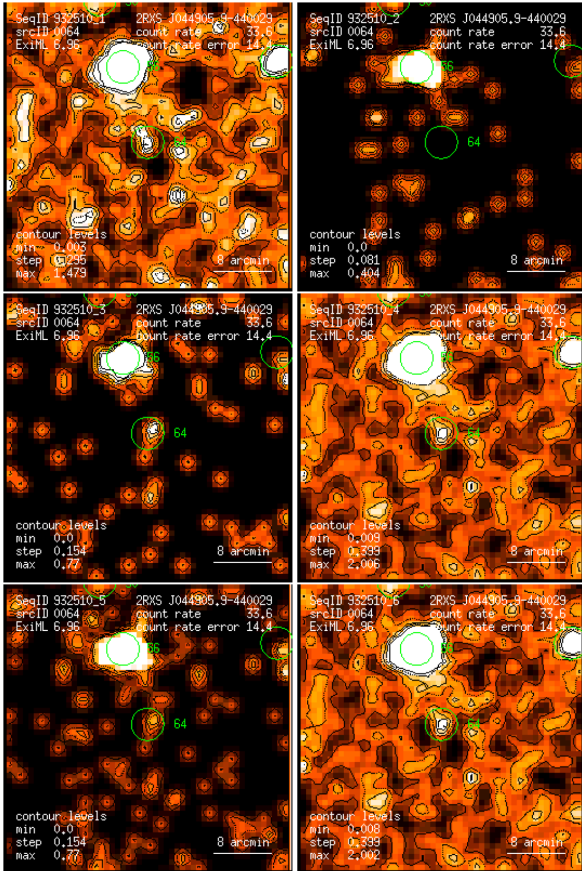
Figure 64: RASS 932510: detection 0064: band rate images, Gaussian filter: (1) PSPC channels 11 – 41, (2) 52 – 90, (3) 91 – 201, (4) 11 – 235, (5) 52 – 201, (6) 11 – 201. Broad band rates in counts/ks. Band rate contour levels in counts/ks/arcmin 2 .
