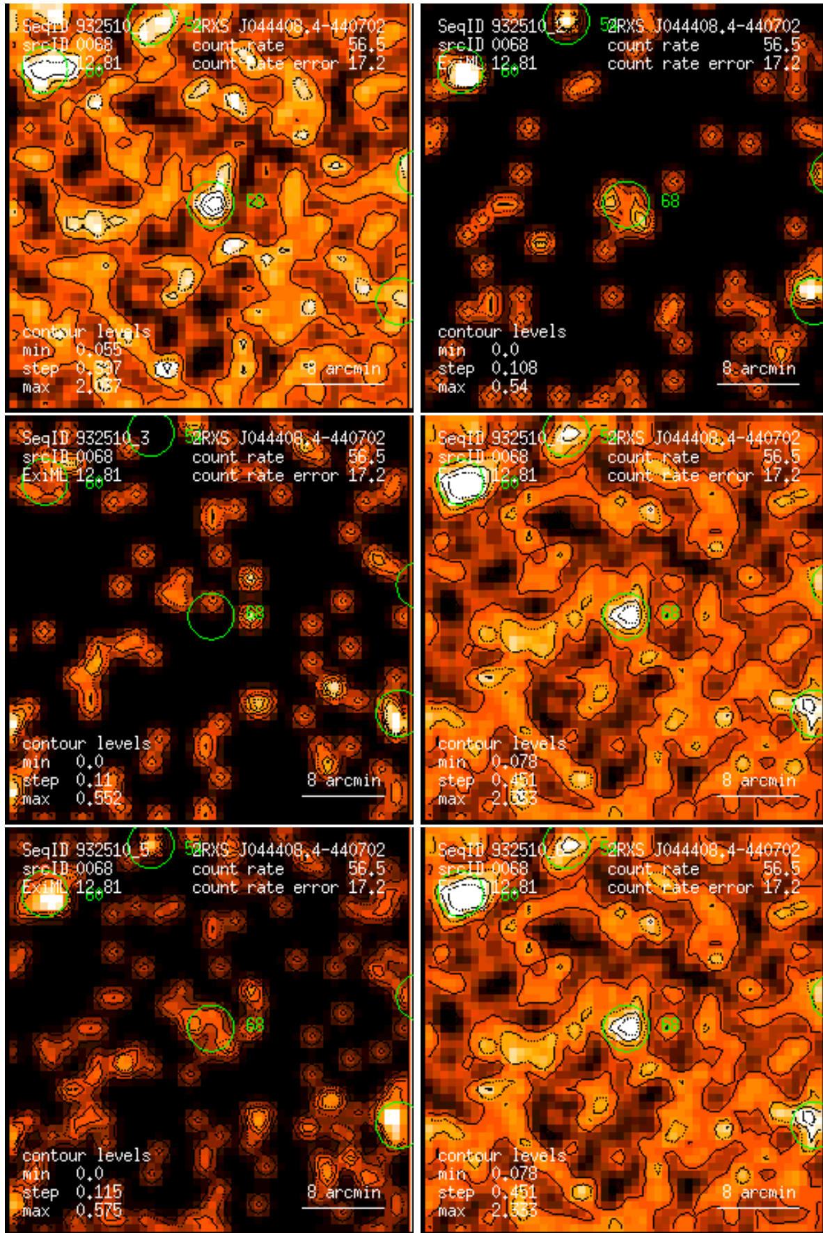
Figure 68: RASS 932510: detection 0068: band rate images, Gaussian filter: (1) PSPC channels 11 – 41, (2) 52 – 90, (3) 91 – 201, (4) 11 – 235, (5) 52 – 201, (6) 11 – 201. Broad band rates in counts/ks. Band rate contour levels in counts/ks/arcmin 2 .
