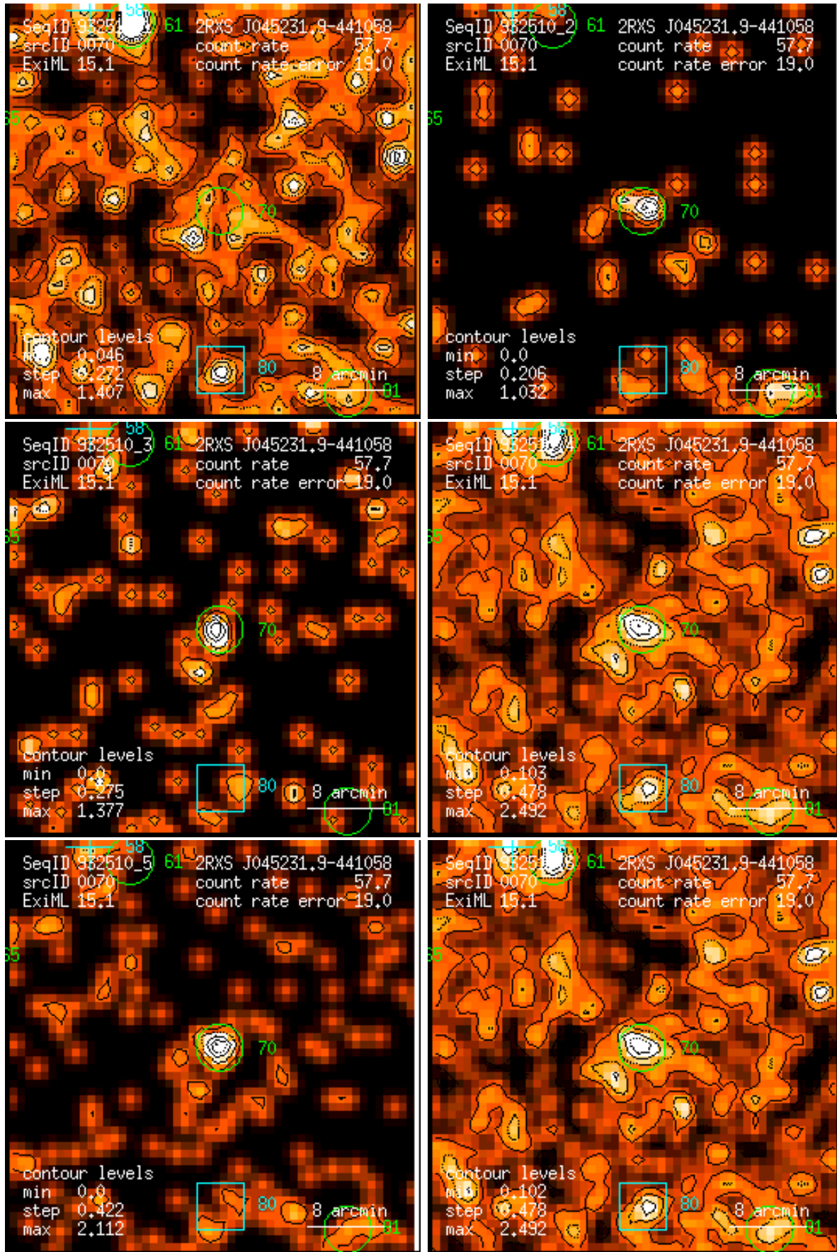
Figure 70: RASS 932510: detection 0070: band rate images, Gaussian filter: (1) PSPC channels 11 – 41, (2) 52 – 90, (3) 91 – 201, (4) 11 – 235, (5) 52 – 201, (6) 11 – 201. Broad band rates in counts/ks. Band rate contour levels in counts/ks/arcmin 2 .
