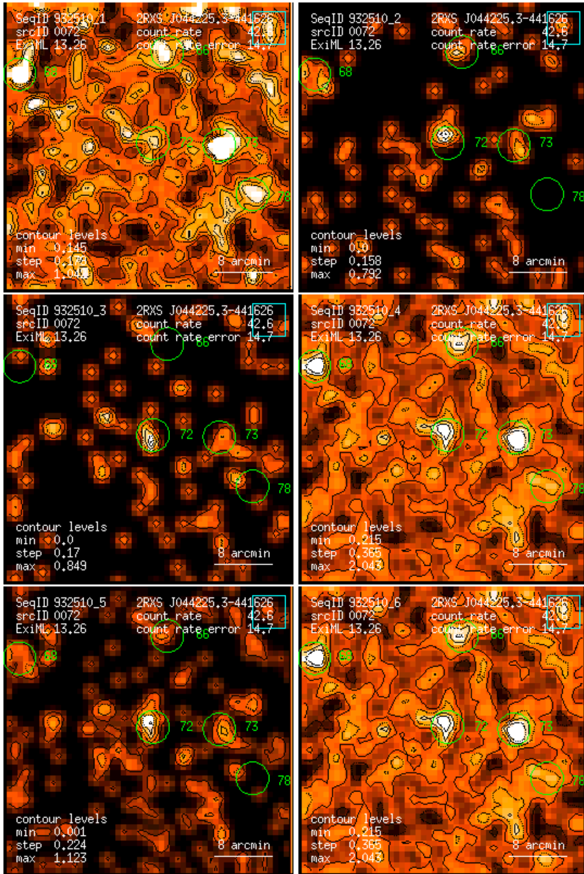
Figure 72: RASS 932510: detection 0072: band rate images, Gaussian filter: (1) PSPC channels 11 – 41, (2) 52 – 90, (3) 91 – 201, (4) 11 – 235, (5) 52 – 201, (6) 11 – 201. Broad band rates in counts/ks. Band rate contour levels in counts/ks/arcmin 2 .
