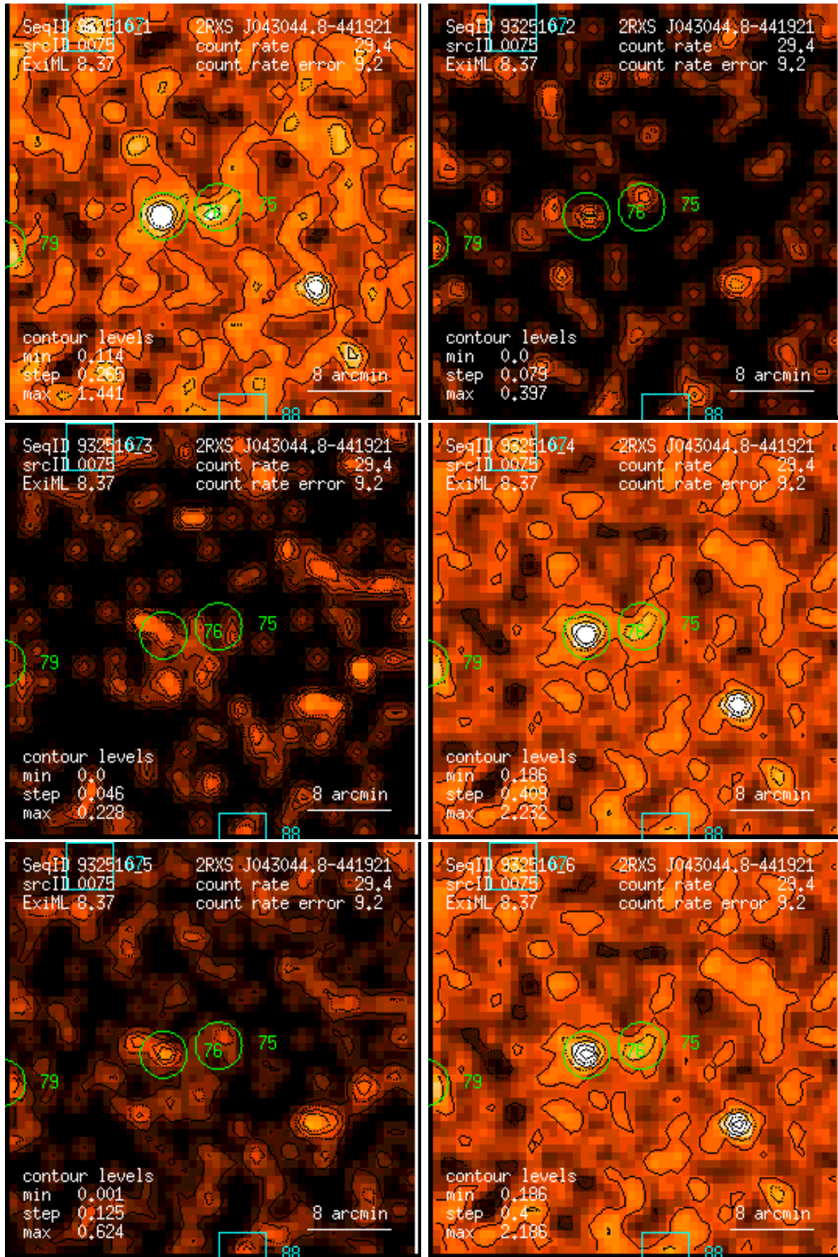
Figure 75: RASS 932510: detection 0075: band rate images, Gaussian filter: (1) PSPC channels 11 – 41, (2) 52 – 90, (3) 91 – 201, (4) 11 – 235, (5) 52 – 201, (6) 11 – 201. Broad band rates in counts/ks. Band rate contour levels in counts/ks/arcmin 2 .
