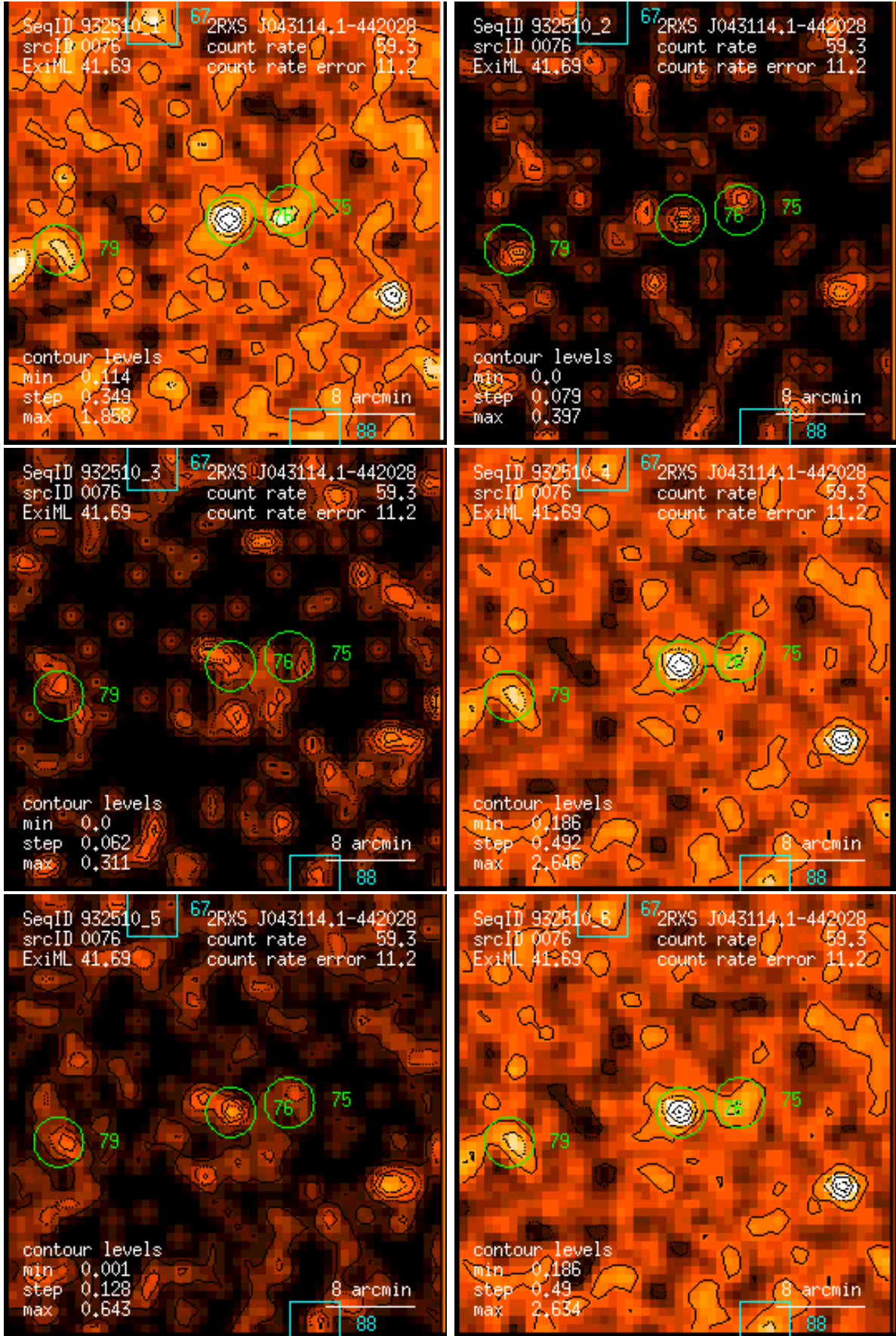
Figure 76: RASS 932510: detection 0076: band rate images, Gaussian filter: (1) PSPC channels 11 – 41, (2) 52 – 90, (3) 91 – 201, (4) 11 – 235, (5) 52 – 201, (6) 11 – 201. Broad band rates in counts/ks. Band rate contour levels in counts/ks/arcmin 2 .
