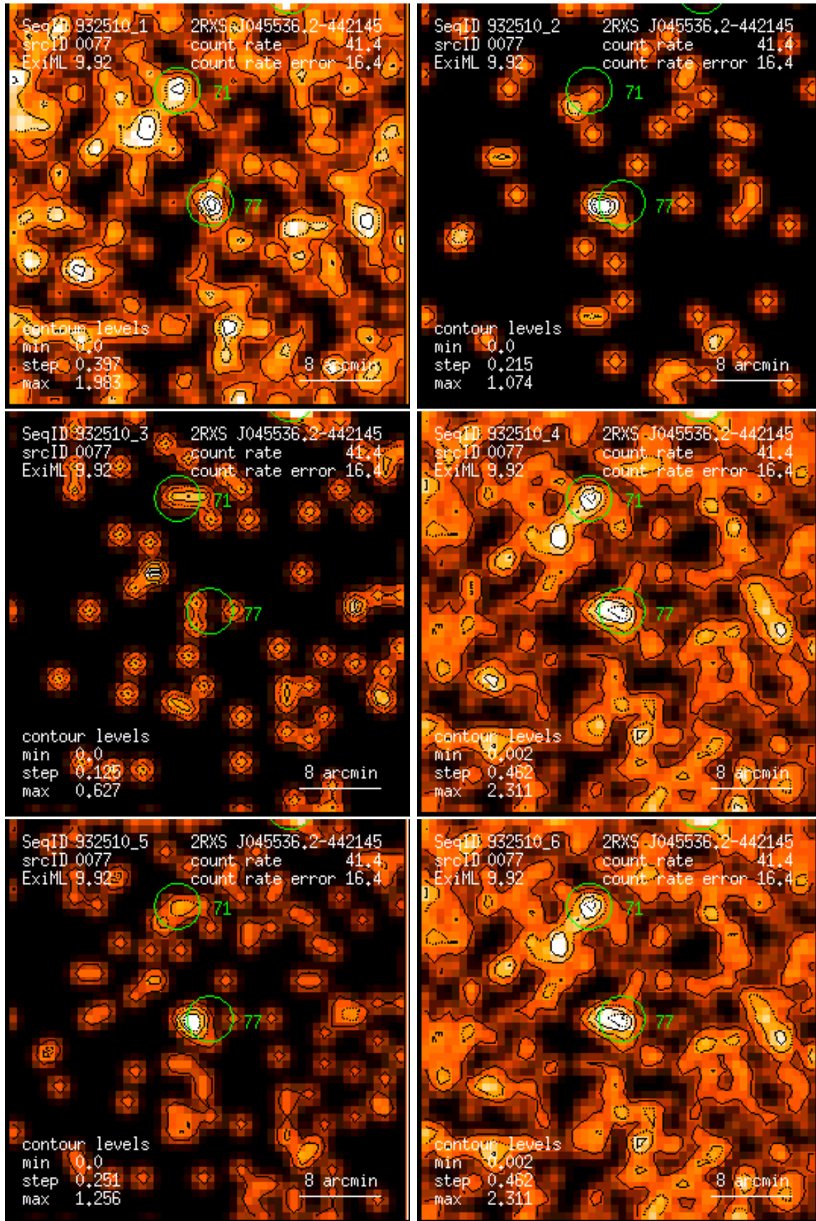
Figure 77: RASS 932510: detection 0077: band rate images, Gaussian filter: (1) PSPC channels 11 – 41, (2) 52 – 90, (3) 91 – 201, (4) 11 – 235, (5) 52 – 201, (6) 11 – 201. Broad band rates in counts/ks. Band rate contour levels in counts/ks/arcmin 2 .
