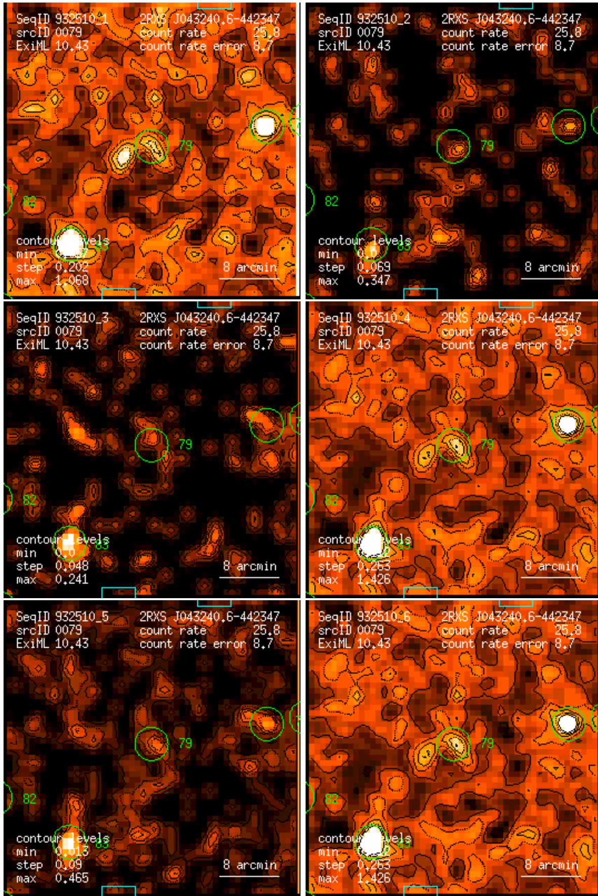
Figure 79: RASS 932510: detection 0079: band rate images, Gaussian filter: (1) PSPC channels 11 – 41, (2) 52 – 90, (3) 91 – 201, (4) 11 – 235, (5) 52 – 201, (6) 11 – 201. Broad band rates in counts/ks. Band rate contour levels in counts/ks/arcmin 2 .
