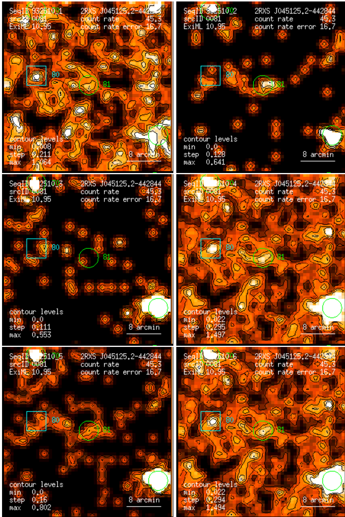
Figure 81: RASS 932510: detection 0081: band rate images, Gaussian filter: (1) PSPC channels 11 – 41, (2) 52 – 90, (3) 91 – 201, (4) 11 – 235, (5) 52 – 201, (6) 11 – 201. Broad band rates in counts/ks. Band rate contour levels in counts/ks/arcmin 2 .
