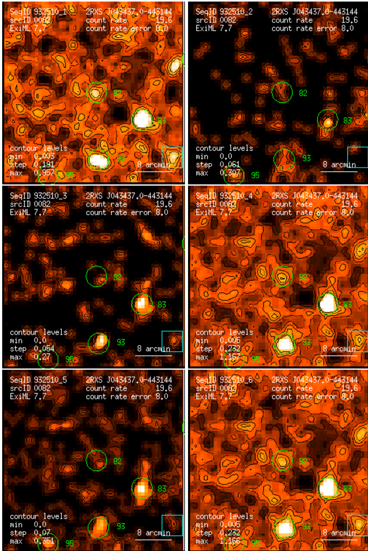
Figure 82: RASS 932510: detection 0082: band rate images, Gaussian filter: (1) PSPC channels 11 – 41, (2) 52 – 90, (3) 91 – 201, (4) 11 – 235, (5) 52 – 201, (6) 11 – 201. Broad band rates in counts/ks. Band rate contour levels in counts/ks/arcmin 2 .
