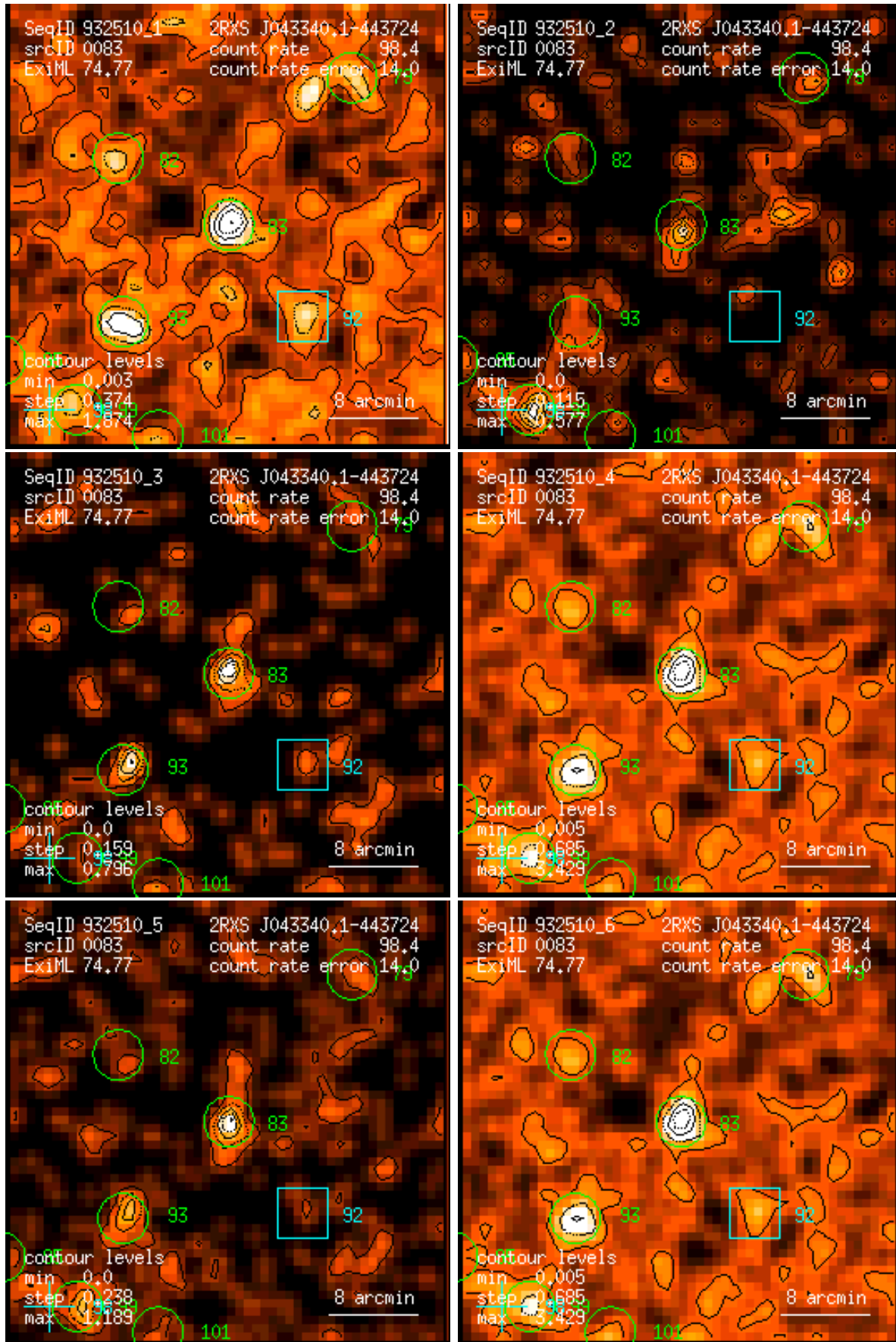
Figure 83: RASS 932510: detection 0083: band rate images, Gaussian filter: (1) PSPC channels 11 – 41, (2) 52 – 90, (3) 91 – 201, (4) 11 – 235, (5) 52 – 201, (6) 11 – 201. Broad band rates in counts/ks. Band rate contour levels in counts/ks/arcmin 2 .
