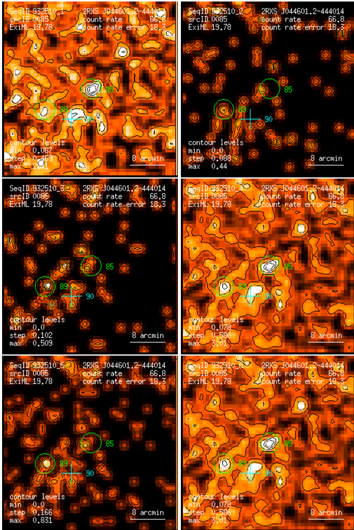
Figure 85: RASS 932510: detection 0085: band rate images, Gaussian filter: (1) PSPC channels 11 – 41, (2) 52 – 90, (3) 91 – 201, (4) 11 – 235, (5) 52 – 201, (6) 11 – 201. Broad band rates in counts/ks. Band rate contour levels in counts/ks/arcmin 2 .
