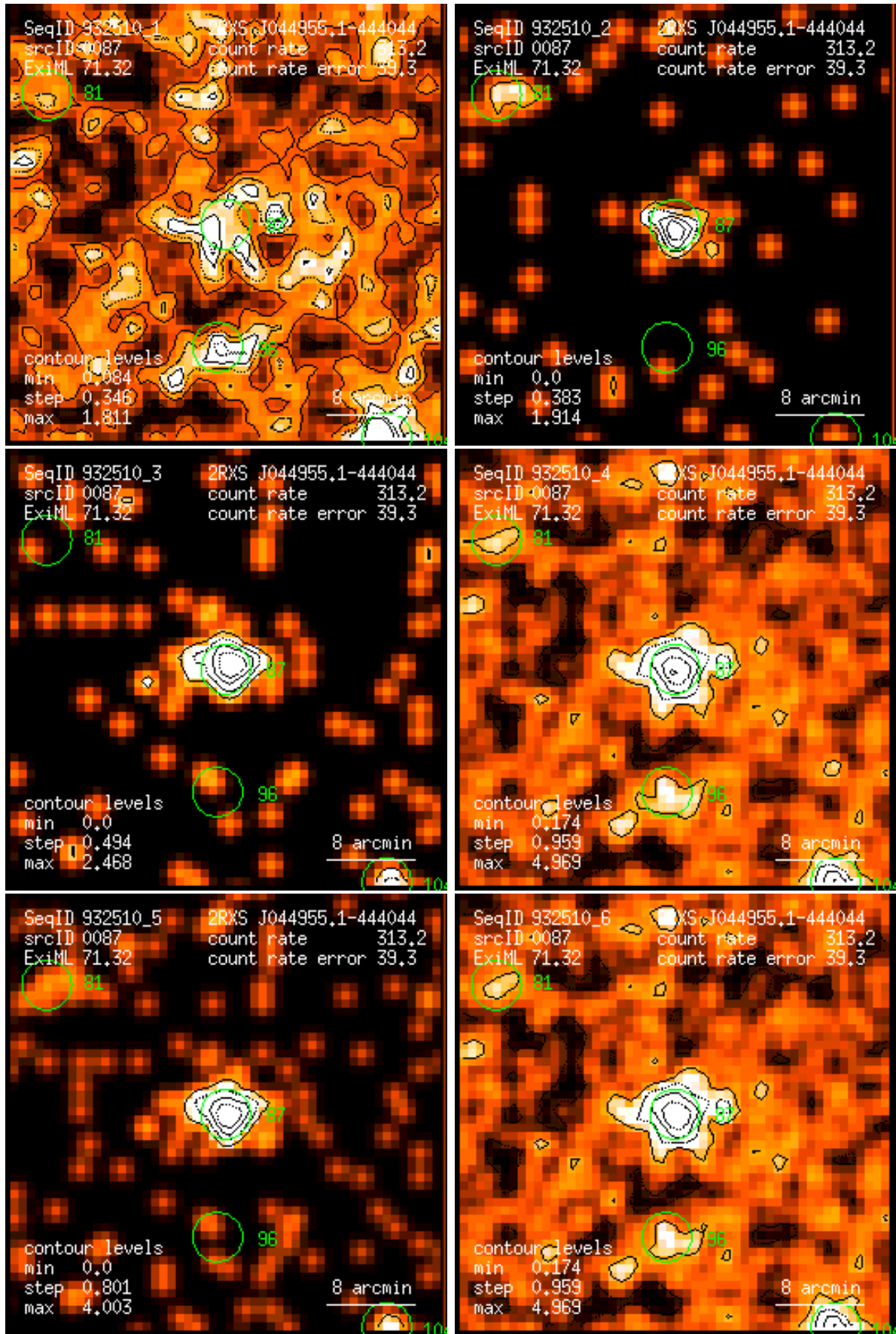
Figure 87: RASS 932510: detection 0087: band rate images, Gaussian filter: (1) PSPC channels 11 – 41, (2) 52 – 90, (3) 91 – 201, (4) 11 – 235, (5) 52 – 201, (6) 11 – 201. Broad band rates in counts/ks. Band rate contour levels in counts/ks/arcmin 2 .
