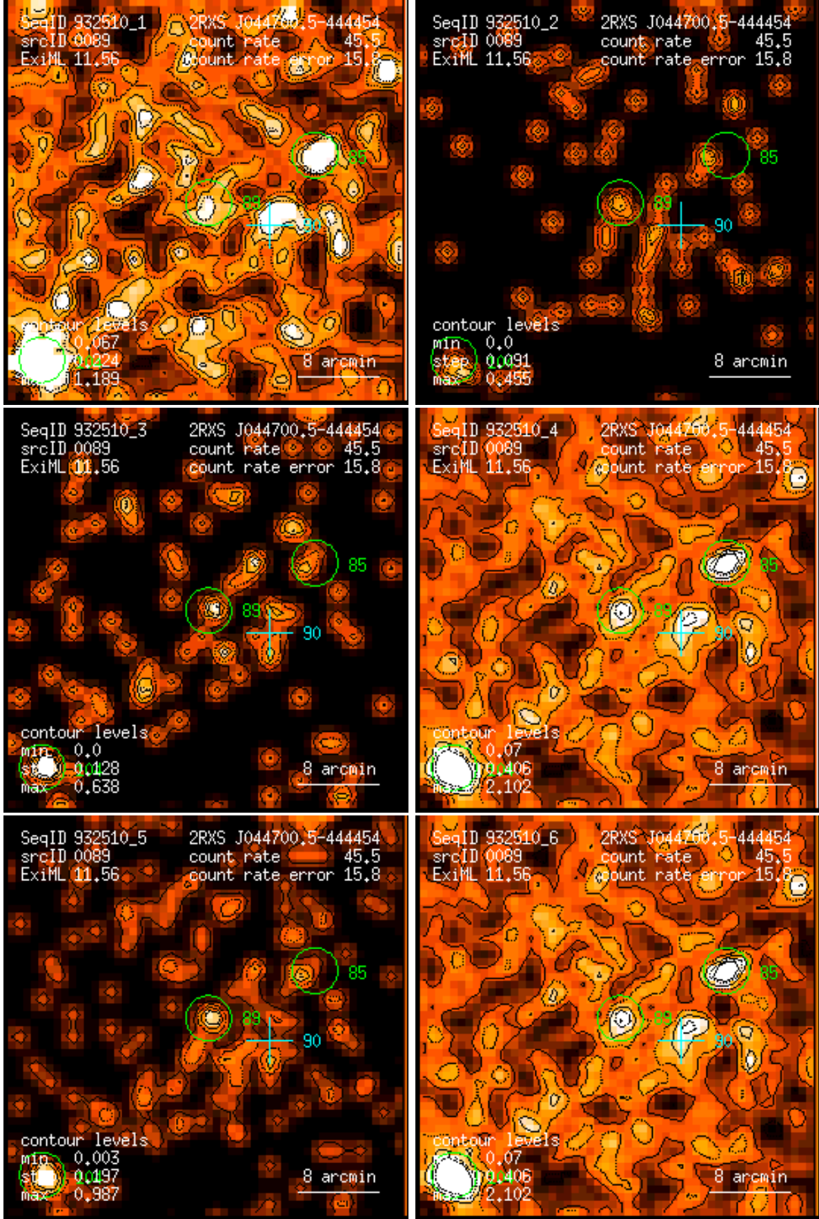
Figure 89: RASS 932510: detection 0089: band rate images, Gaussian filter: (1) PSPC channels 11 – 41, (2) 52 – 90, (3) 91 – 201, (4) 11 – 235, (5) 52 – 201, (6) 11 – 201. Broad band rates in counts/ks. Band rate contour levels in counts/ks/arcmin 2 .
