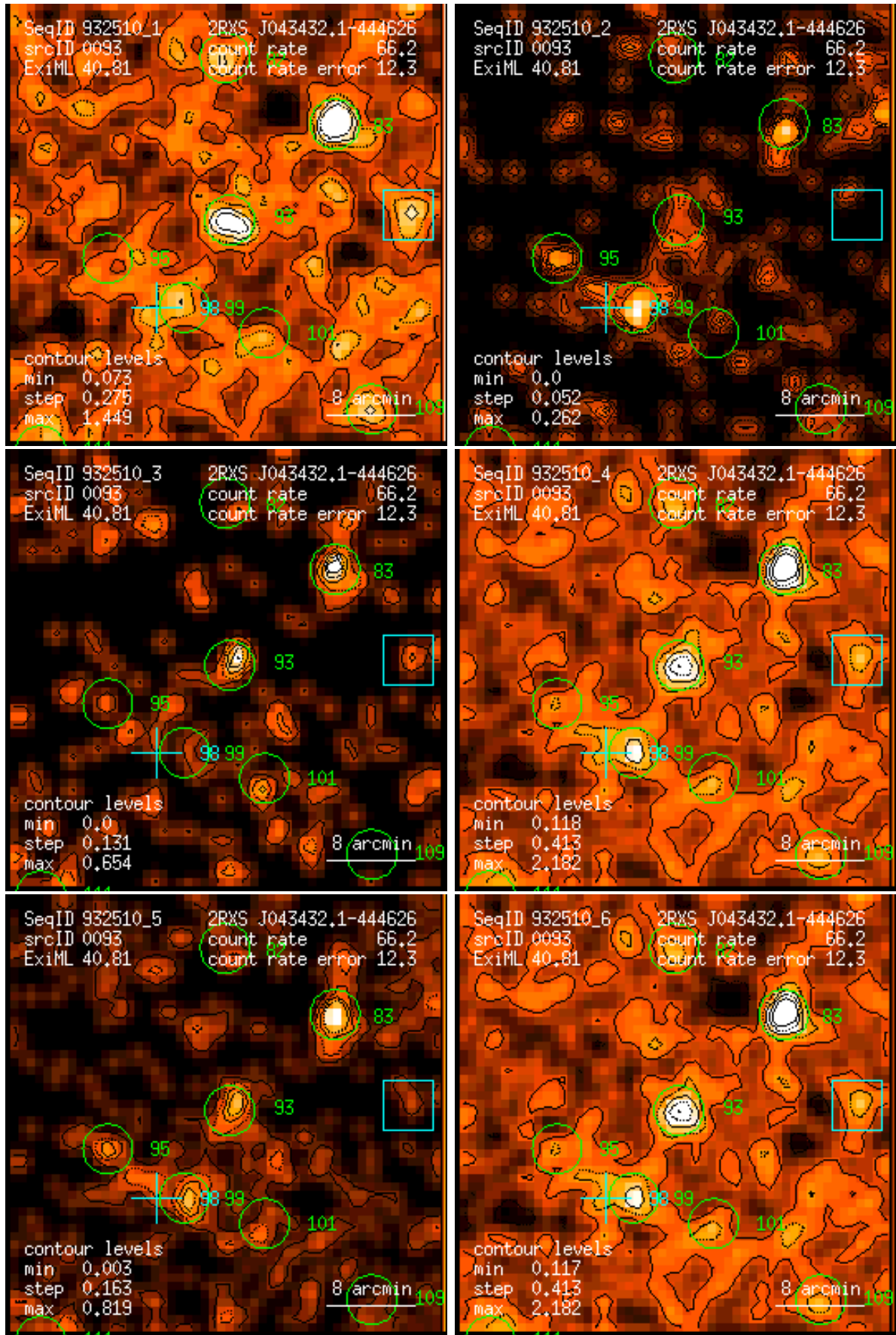
Figure 93: RASS 932510: detection 0093: band rate images, Gaussian filter: (1) PSPC channels 11 – 41, (2) 52 – 90, (3) 91 – 201, (4) 11 – 235, (5) 52 – 201, (6) 11 – 201. Broad band rates in counts/ks. Band rate contour levels in counts/ks/arcmin 2 .
