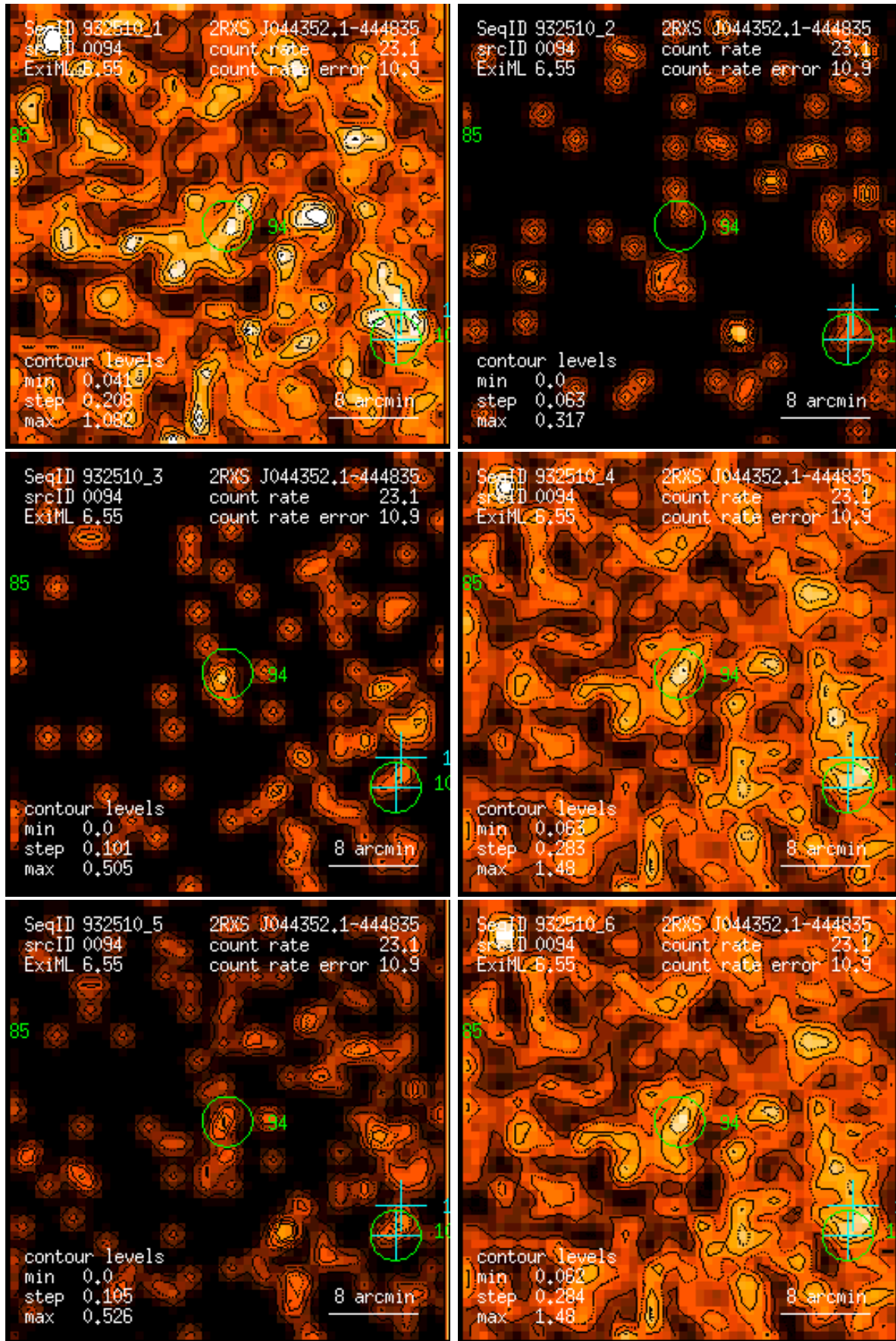
Figure 94: RASS 932510: detection 0094: band rate images, Gaussian filter: (1) PSPC channels 11 – 41, (2) 52 – 90, (3) 91 – 201, (4) 11 – 235, (5) 52 – 201, (6) 11 – 201. Broad band rates in counts/ks. Band rate contour levels in counts/ks/arcmin 2 .
