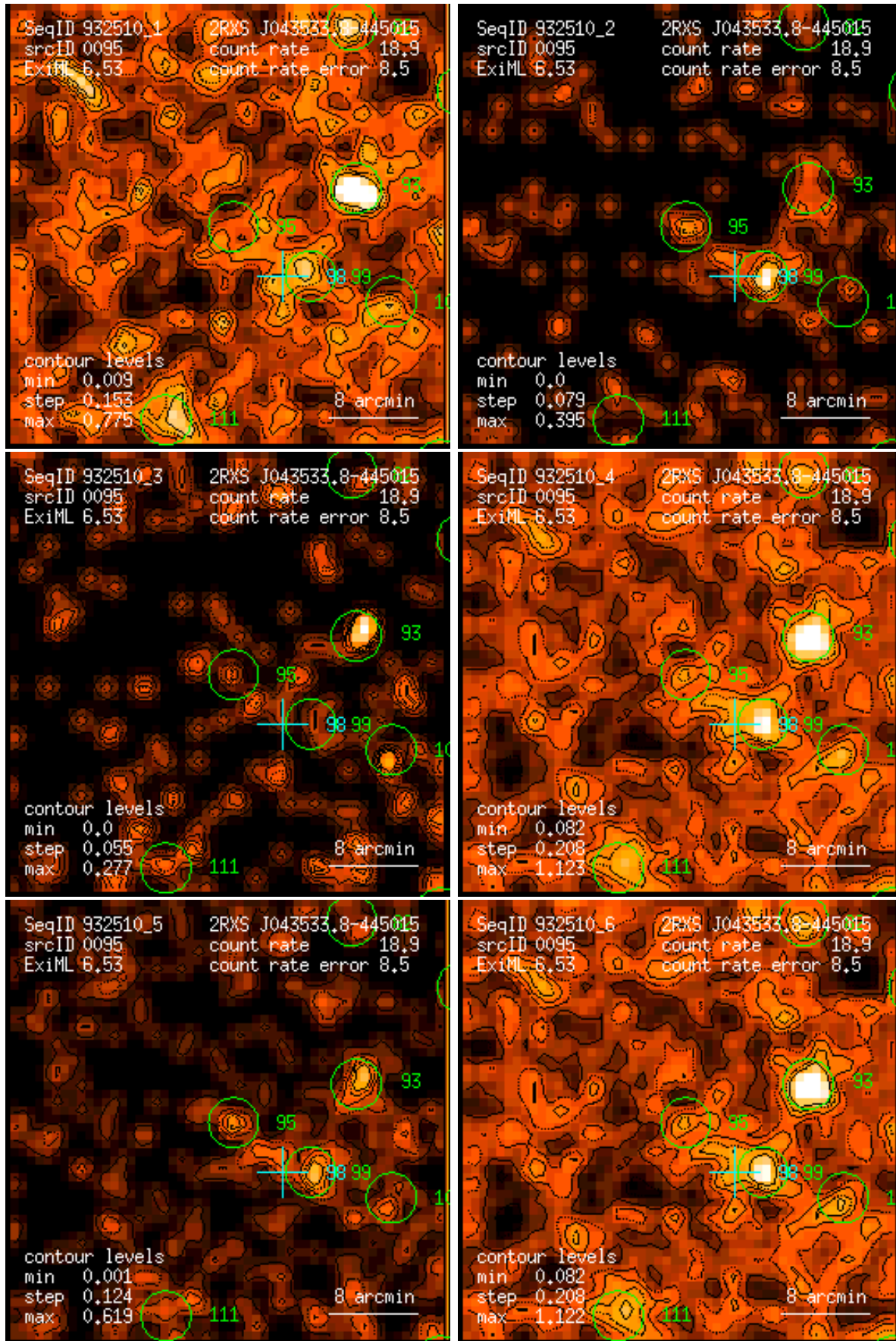
Figure 95: RASS 932510: detection 0095: band rate images, Gaussian filter: (1) PSPC channels 11 – 41, (2) 52 – 90, (3) 91 – 201, (4) 11 – 235, (5) 52 – 201, (6) 11 – 201. Broad band rates in counts/ks. Band rate contour levels in counts/ks/arcmin 2 .
