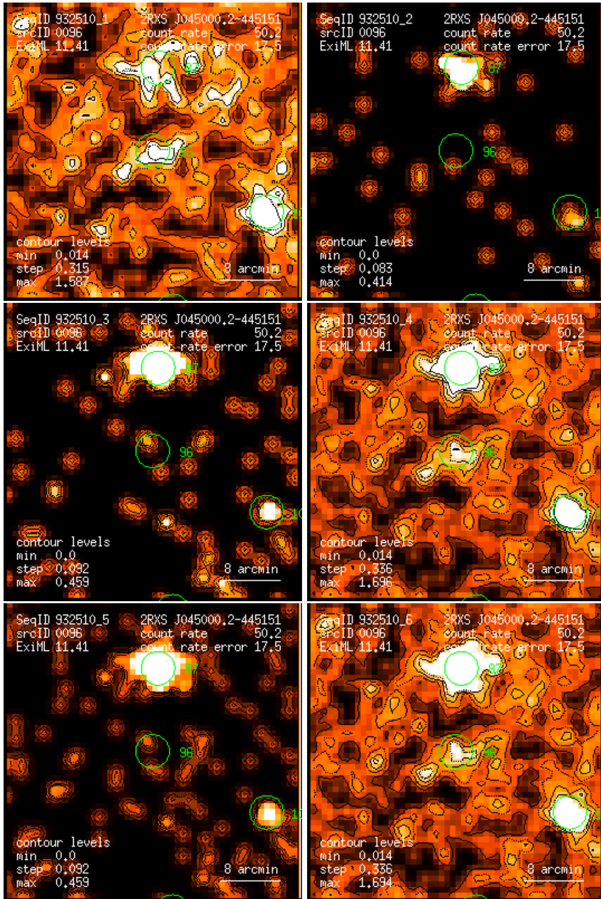
Figure 96: RASS 932510: detection 0096: band rate images, Gaussian filter: (1) PSPC channels 11 – 41, (2) 52 – 90, (3) 91 – 201, (4) 11 – 235, (5) 52 – 201, (6) 11 – 201. Broad band rates in counts/ks. Band rate contour levels in counts/ks/arcmin 2 .
