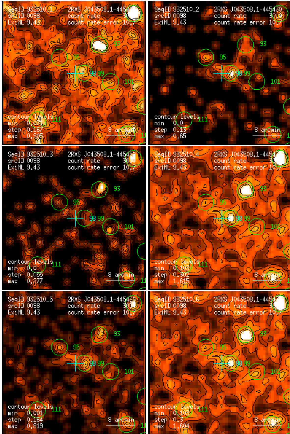
Figure 98: RASS 932510: detection 0098: band rate images, Gaussian filter: (1) PSPC channels 11 – 41, (2) 52 – 90, (3) 91 – 201, (4) 11 – 235, (5) 52 – 201, (6) 11 – 201. Broad band rates in counts/ks. Band rate contour levels in counts/ks/arcmin 2 .
