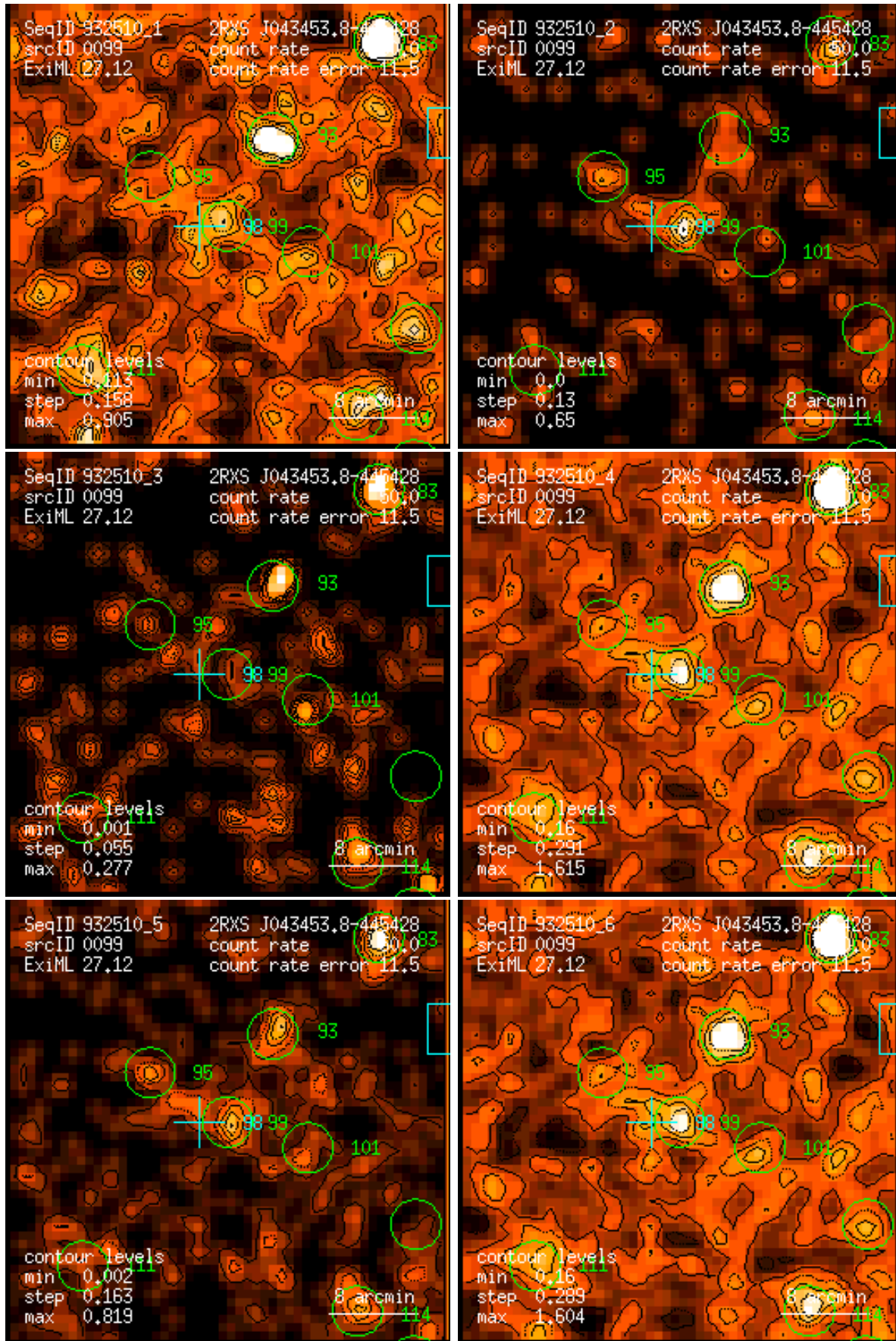
Figure 99: RASS 932510: detection 0099: band rate images, Gaussian filter: (1) PSPC channels 11 – 41, (2) 52 – 90, (3) 91 – 201, (4) 11 – 235, (5) 52 – 201, (6) 11 – 201. Broad band rates in counts/ks. Band rate contour levels in counts/ks/arcmin 2 .
