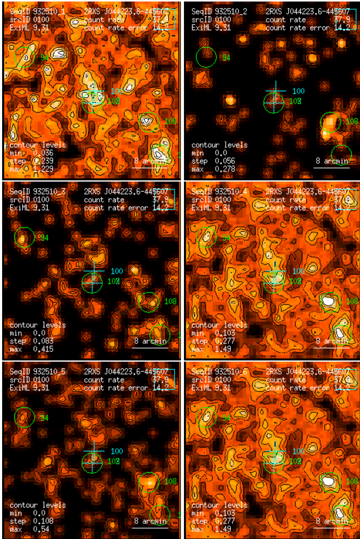
Figure 100: RASS 932510: detection 0100: band rate images, Gaussian filter: (1) PSPC channels 11 – 41, (2) 52 – 90, (3) 91 – 201, (4) 11 – 235, (5) 52 – 201, (6) 11 – 201. Broad band rates in counts/ks. Band rate contour levels in counts/ks/arcmin 2 .
