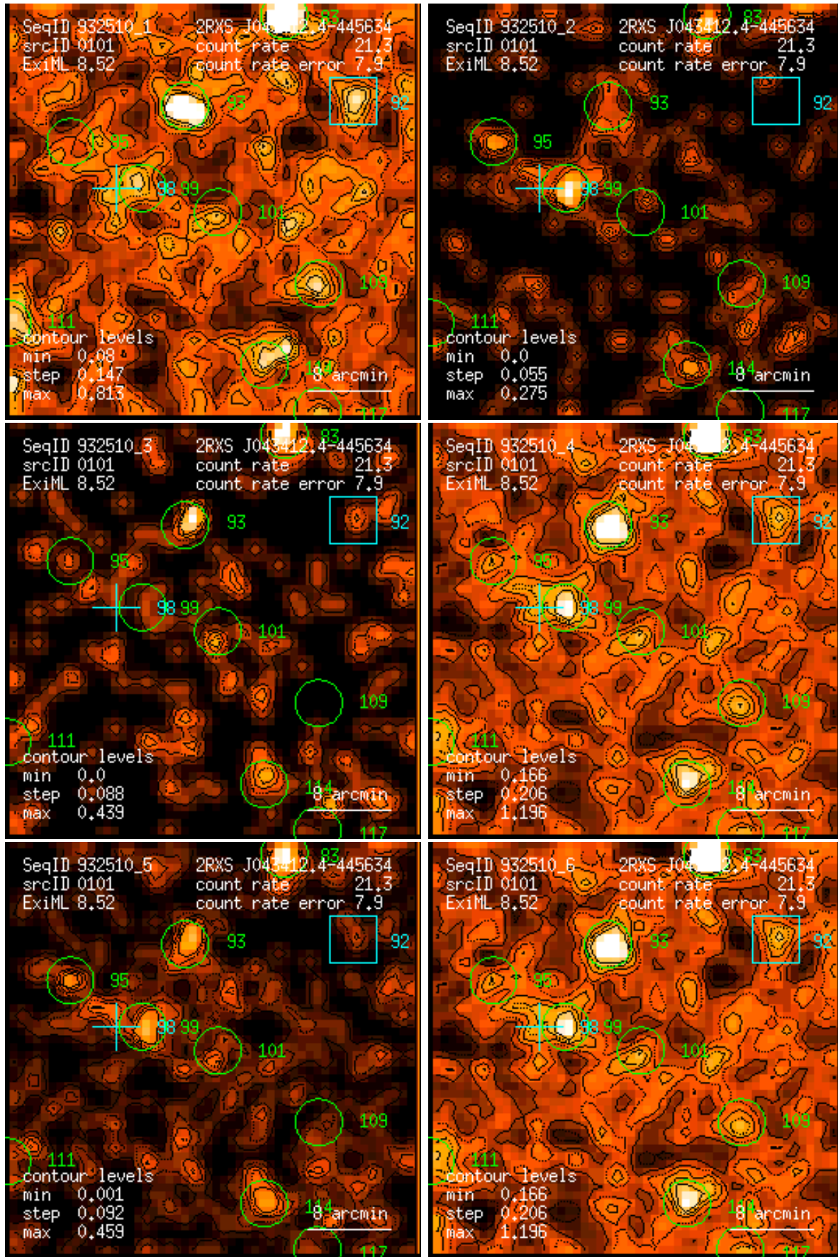
Figure 101: RASS 932510: detection 0101: band rate images, Gaussian filter: (1) PSPC channels 11 – 41, (2) 52 – 90, (3) 91 – 201, (4) 11 – 235, (5) 52 – 201, (6) 11 – 201. Broad band rates in counts/ks. Band rate contour levels in counts/ks/arcmin 2 .
