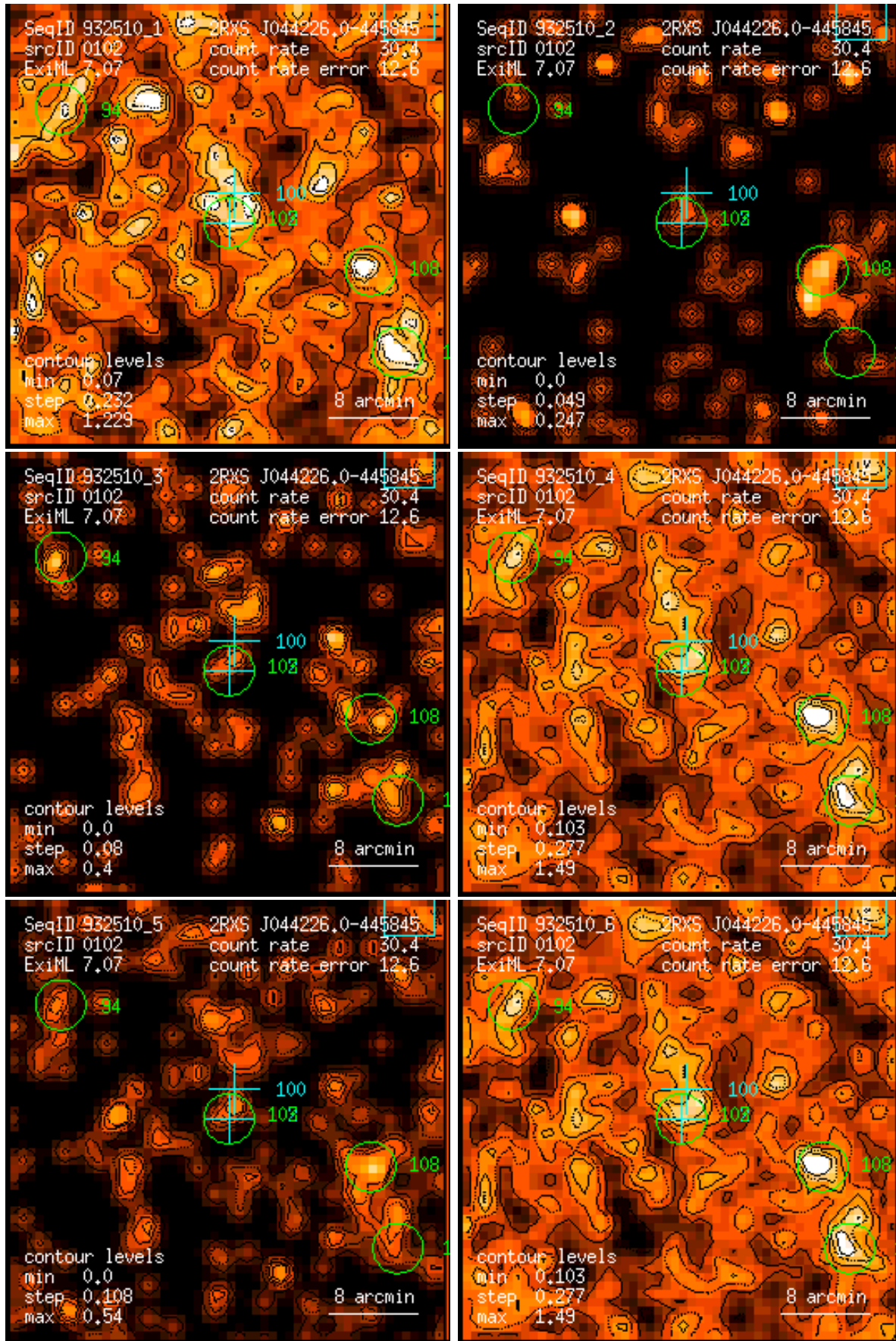
Figure 102: RASS 932510: detection 0102: band rate images, Gaussian filter: (1) PSPC channels 11 – 41, (2) 52 – 90, (3) 91 – 201, (4) 11 – 235, (5) 52 – 201, (6) 11 – 201. Broad band rates in counts/ks. Band rate contour levels in counts/ks/arcmin 2 .
