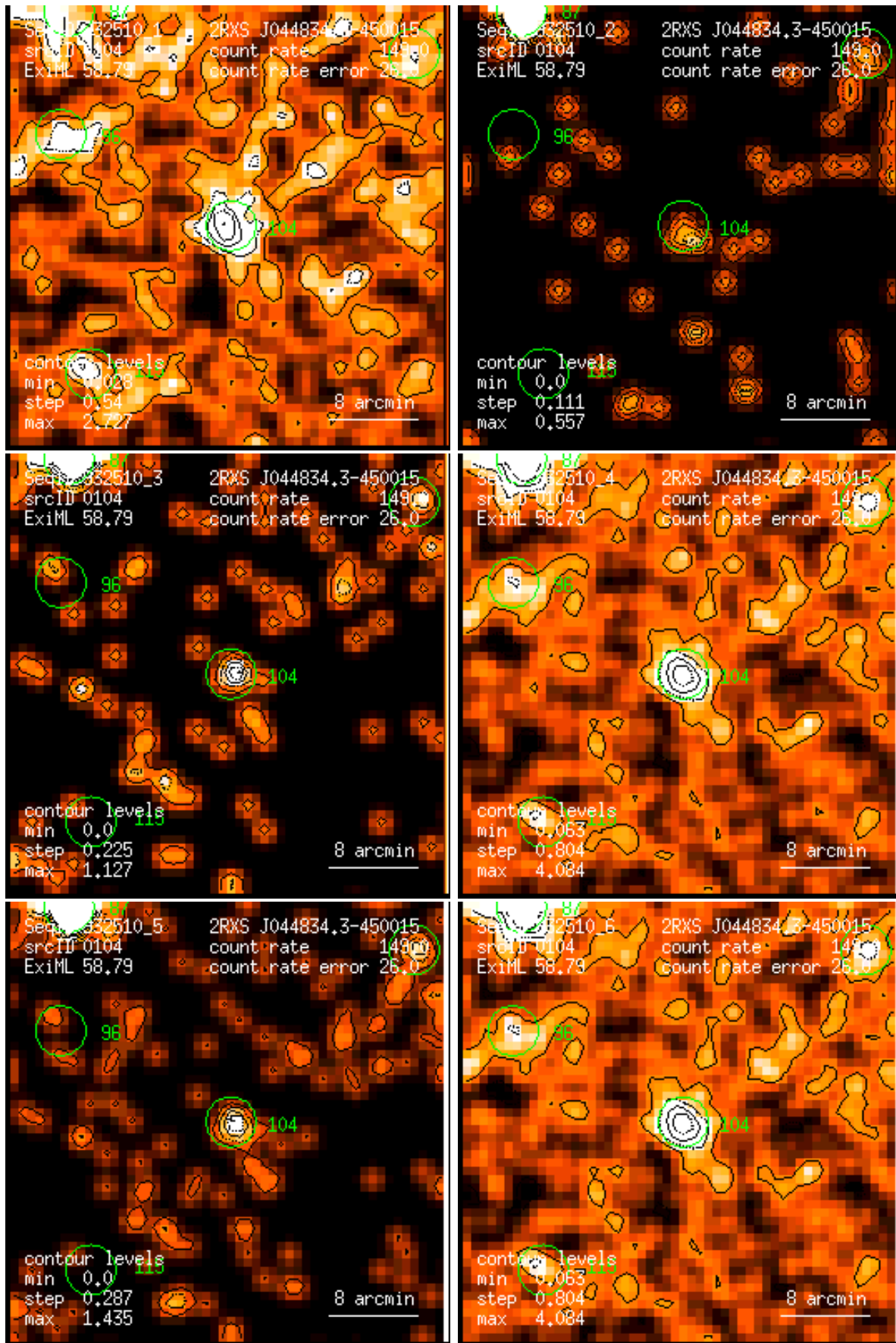
Figure 104: RASS 932510: detection 0104: band rate images, Gaussian filter: (1) PSPC channels 11 – 41, (2) 52 – 90, (3) 91 – 201, (4) 11 – 235, (5) 52 – 201, (6) 11 – 201. Broad band rates in counts/ks. Band rate contour levels in counts/ks/arcmin 2 .
