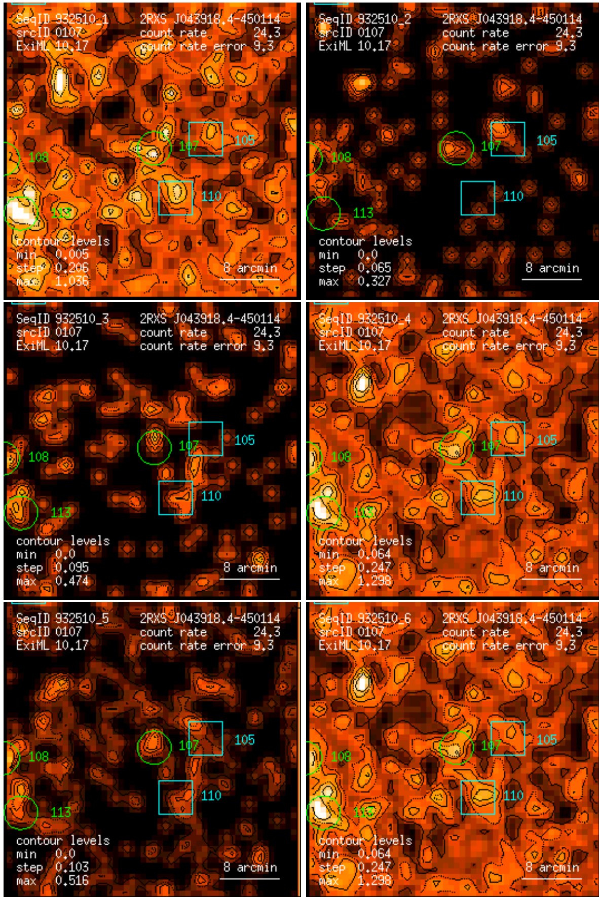
Figure 107: RASS 932510: detection 0107: band rate images, Gaussian filter: (1) PSPC channels 11 – 41, (2) 52 – 90, (3) 91 – 201, (4) 11 – 235, (5) 52 – 201, (6) 11 – 201. Broad band rates in counts/ks. Band rate contour levels in counts/ks/arcmin 2 .
