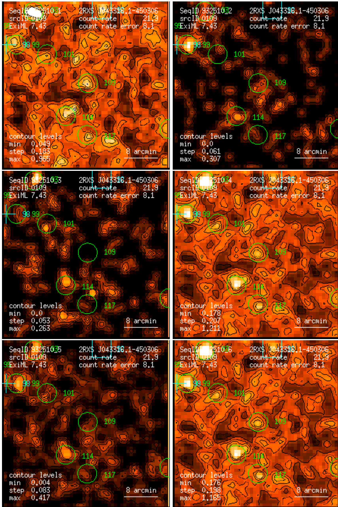
Figure 109: RASS 932510: detection 0109: band rate images, Gaussian filter: (1) PSPC channels 11 – 41, (2) 52 – 90, (3) 91 – 201, (4) 11 – 235, (5) 52 – 201, (6) 11 – 201. Broad band rates in counts/ks. Band rate contour levels in counts/ks/arcmin 2 .
