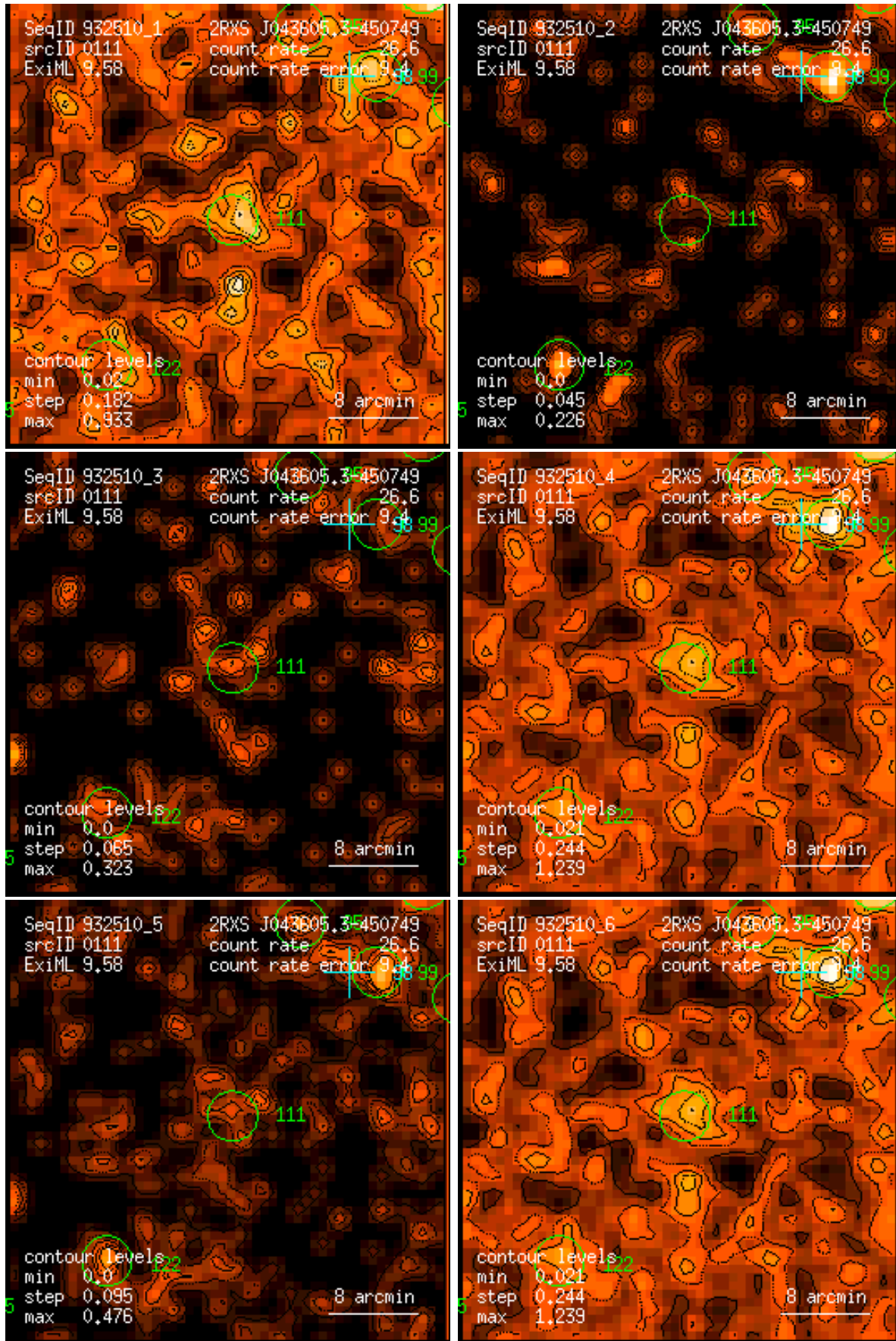
Figure 111: RASS 932510: detection 0111: band rate images, Gaussian filter: (1) PSPC channels 11 – 41, (2) 52 – 90, (3) 91 – 201, (4) 11 – 235, (5) 52 – 201, (6) 11 – 201. Broad band rates in counts/ks. Band rate contour levels in counts/ks/arcmin 2 .
