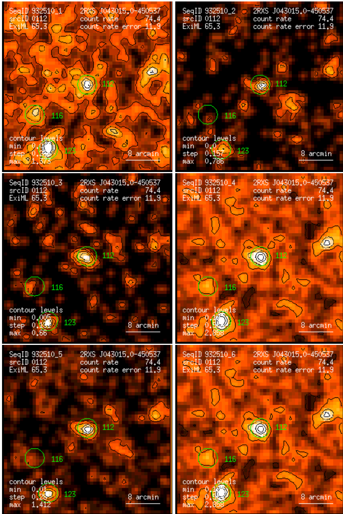
Figure 112: RASS 932510: detection 0112: band rate images, Gaussian filter: (1) PSPC channels 11 – 41, (2) 52 – 90, (3) 91 – 201, (4) 11 – 235, (5) 52 – 201, (6) 11 – 201. Broad band rates in counts/ks. Band rate contour levels in counts/ks/arcmin 2 .
