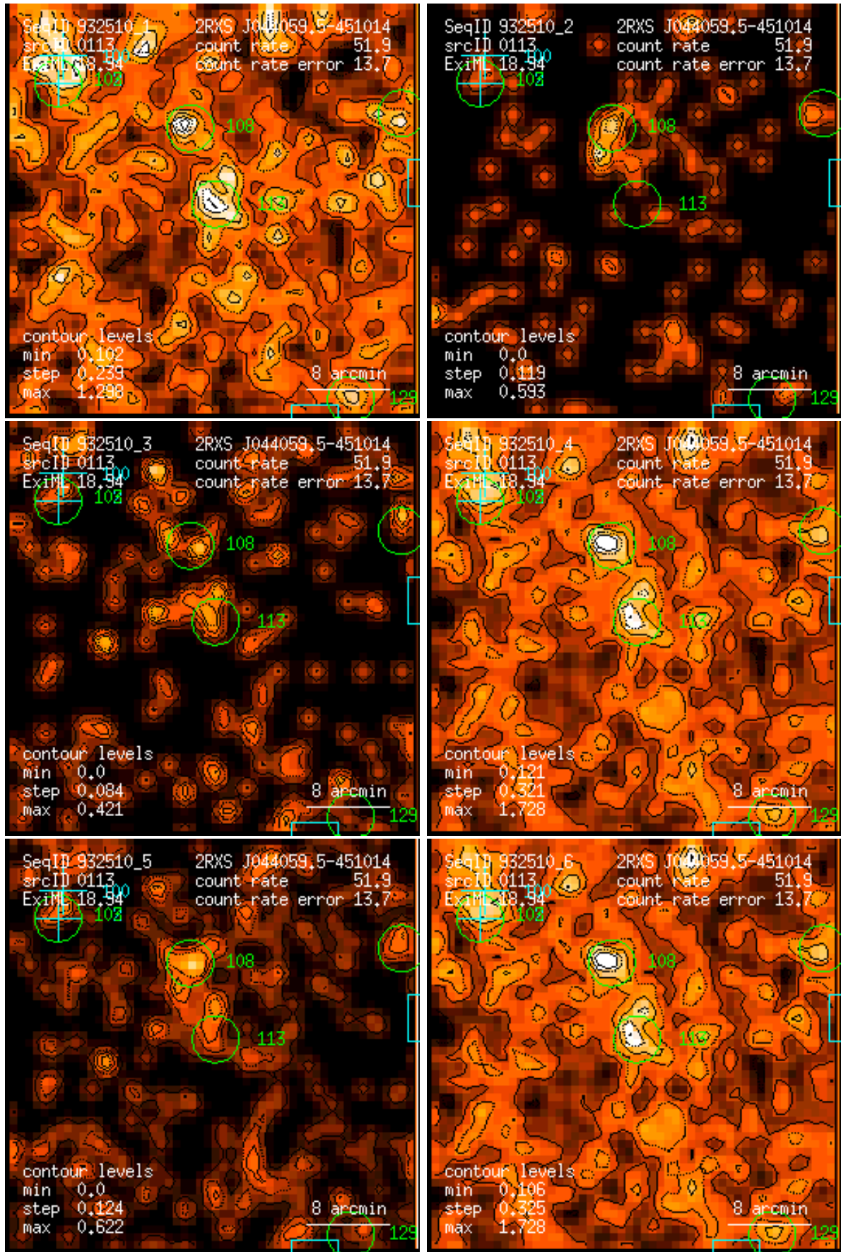
Figure 113: RASS 932510: detection 0113: band rate images, Gaussian filter: (1) PSPC channels 11 – 41, (2) 52 – 90, (3) 91 – 201, (4) 11 – 235, (5) 52 – 201, (6) 11 – 201. Broad band rates in counts/ks. Band rate contour levels in counts/ks/arcmin 2 .
