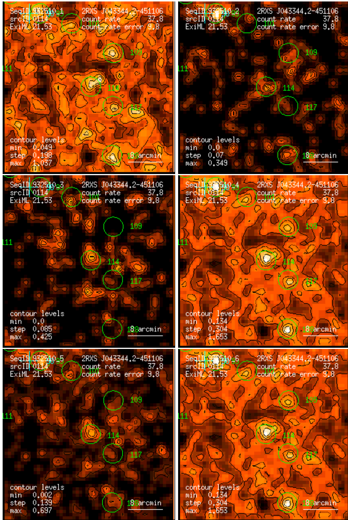
Figure 114: RASS 932510: detection 0114: band rate images, Gaussian filter: (1) PSPC channels 11 – 41, (2) 52 – 90, (3) 91 – 201, (4) 11 – 235, (5) 52 – 201, (6) 11 – 201. Broad band rates in counts/ks. Band rate contour levels in counts/ks/arcmin 2 .
