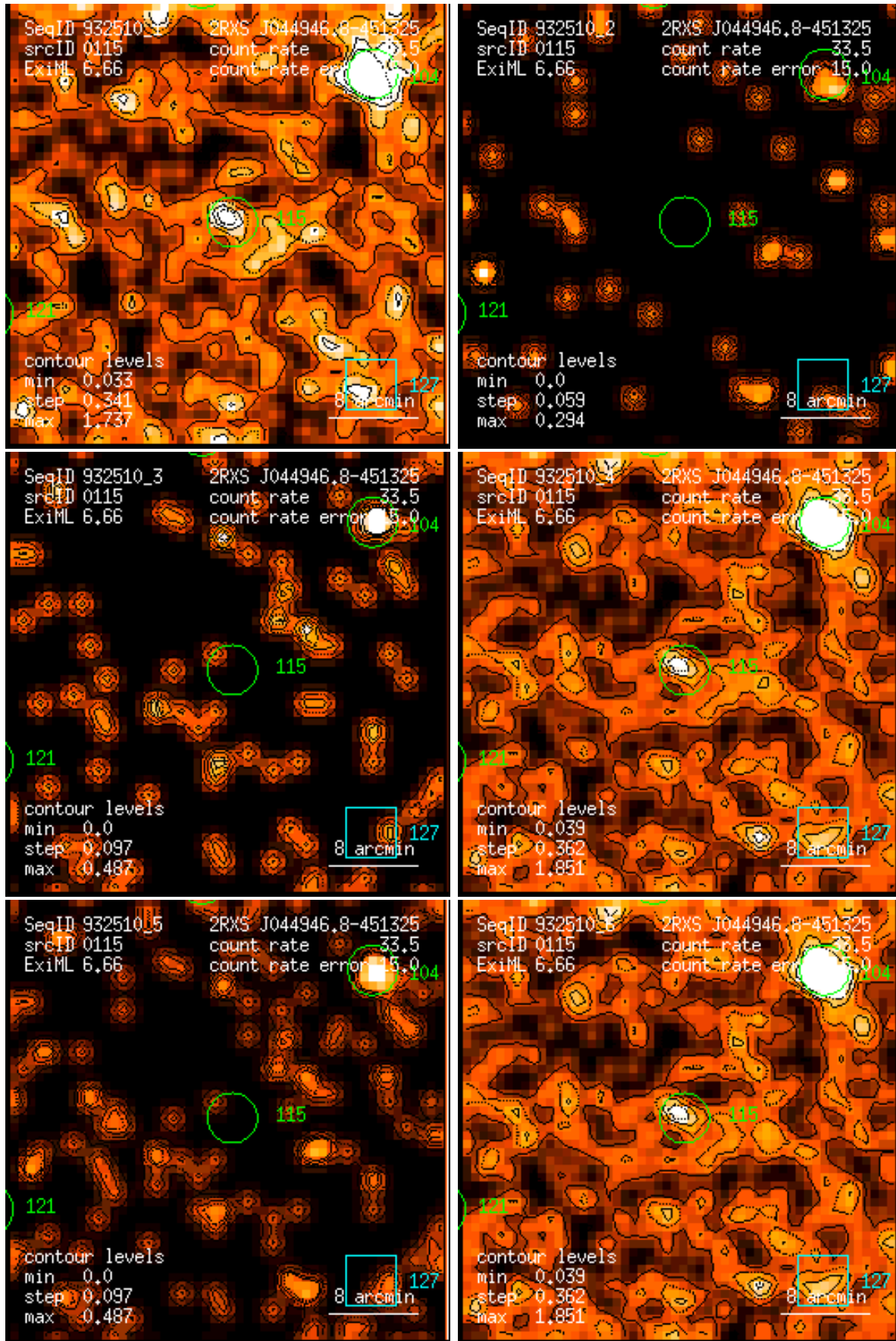
Figure 115: RASS 932510: detection 0115: band rate images, Gaussian filter: (1) PSPC channels 11 – 41, (2) 52 – 90, (3) 91 – 201, (4) 11 – 235, (5) 52 – 201, (6) 11 – 201. Broad band rates in counts/ks. Band rate contour levels in counts/ks/arcmin 2 .
