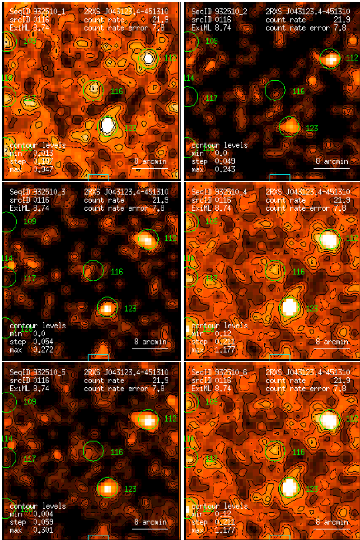
Figure 116: RASS 932510: detection 0116: band rate images, Gaussian filter: (1) PSPC channels 11 – 41, (2) 52 – 90, (3) 91 – 201, (4) 11 – 235, (5) 52 – 201, (6) 11 – 201. Broad band rates in counts/ks. Band rate contour levels in counts/ks/arcmin 2 .
