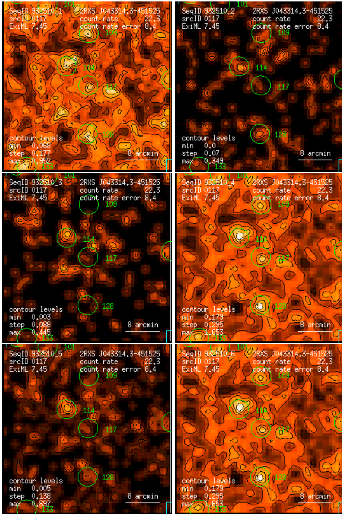
Figure 117: RASS 932510: detection 0117: band rate images, Gaussian filter: (1) PSPC channels 11 – 41, (2) 52 – 90, (3) 91 – 201, (4) 11 – 235, (5) 52 – 201, (6) 11 – 201. Broad band rates in counts/ks. Band rate contour levels in counts/ks/arcmin 2 .
