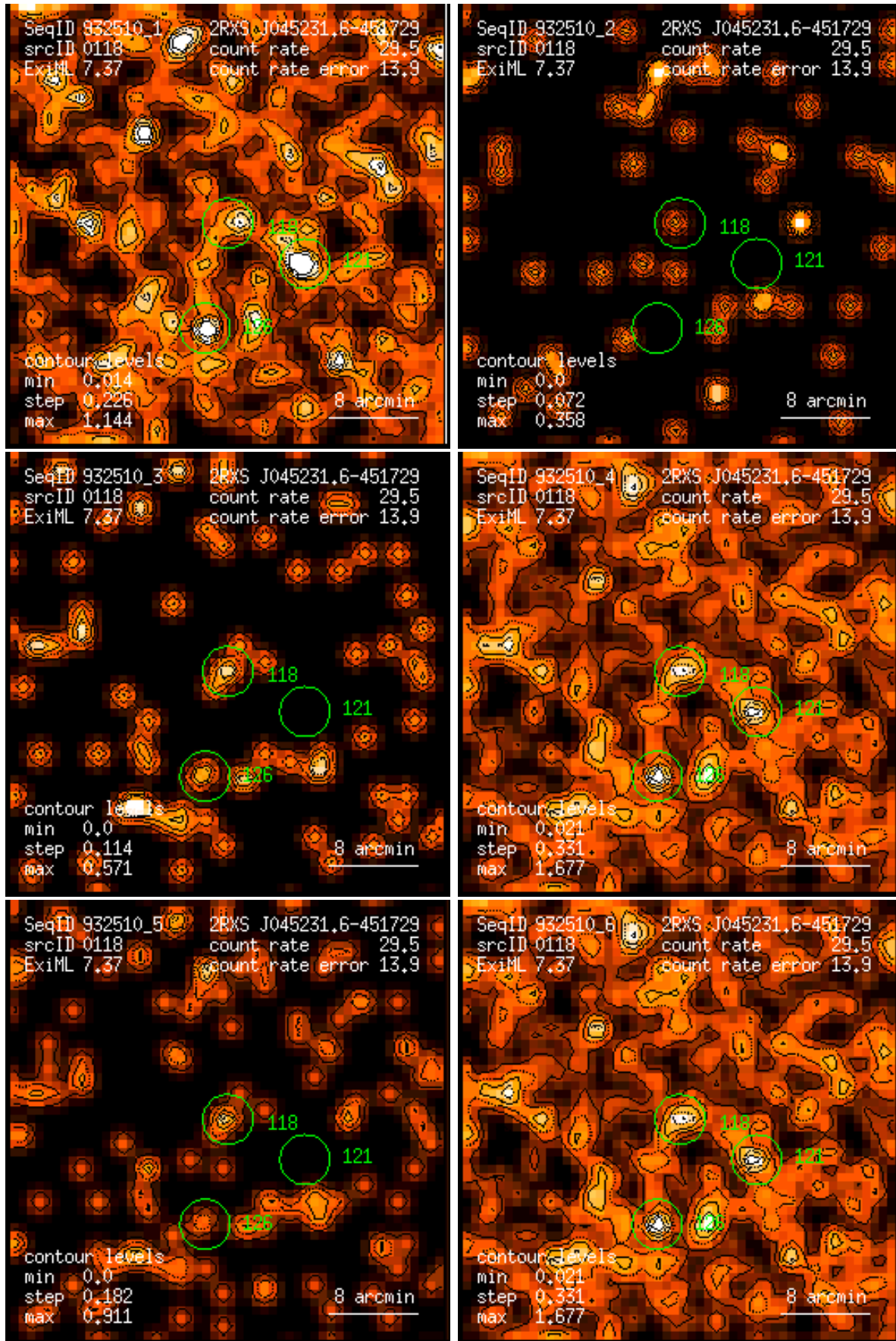
Figure 118: RASS 932510: detection 0118: band rate images, Gaussian filter: (1) PSPC channels 11 – 41, (2) 52 – 90, (3) 91 – 201, (4) 11 – 235, (5) 52 – 201, (6) 11 – 201. Broad band rates in counts/ks. Band rate contour levels in counts/ks/arcmin 2 .
